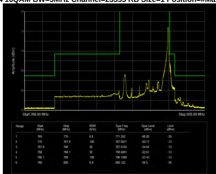
Band14 16QAM BW=5MHz Channel=23355 RB Size=1 Position=#Max Normal
