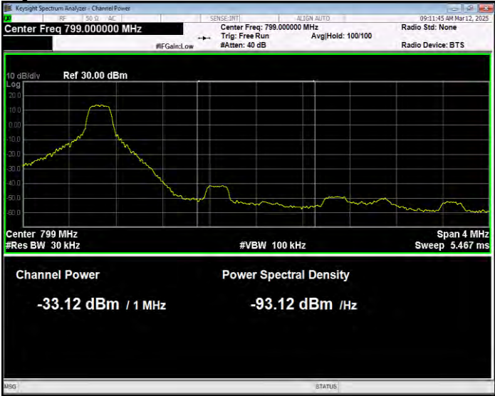
Band14 QPSK BW=10MHz Channel=23330 RB Size=1 Position=#0 Extended
