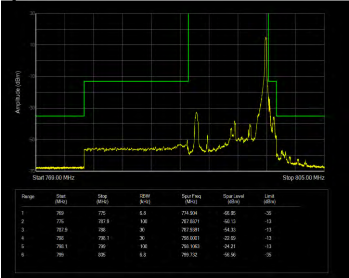
Band14 QPSK BW=5MHz Channel=23355 RB Size=1 Position=#Max Extended
