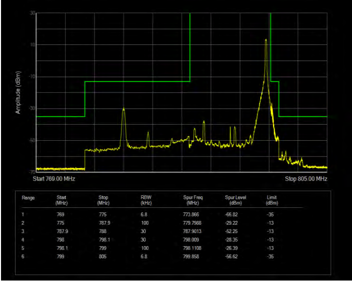
Band14 16QAM BW=10MHz Channel=23330 RB Size=1 Position=#Max Normal
