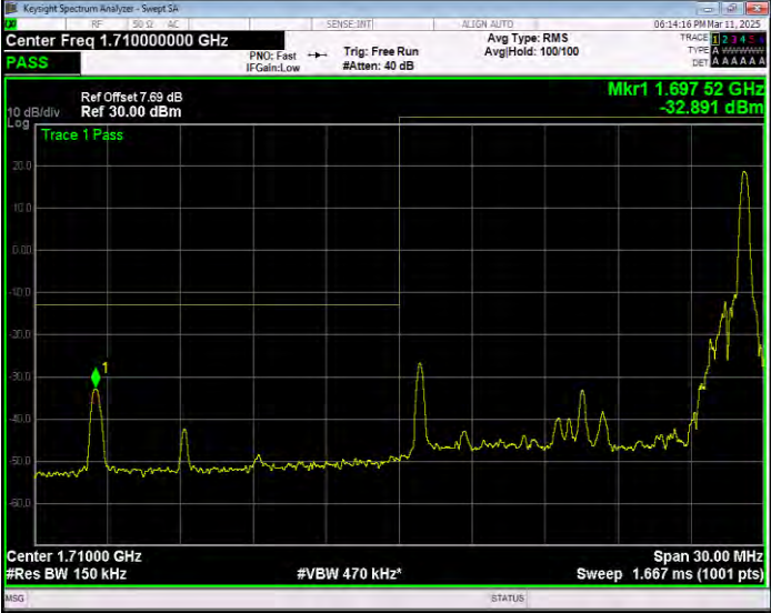
Band4 QPSK BW=15MHz Channel=20025 RB Size=1 Position=#Max Extended
