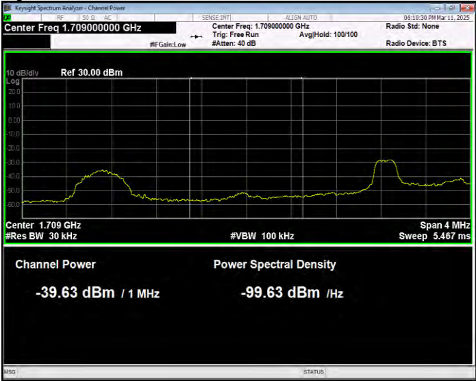
Band4 16QAM BW=3MHz Channel=19965 RB Size=1 Position=#0 Normal
