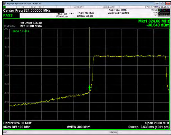
Band5 16QAM BW=10MHz Channel=20600 RB Size=1 Position=#0 Normal
