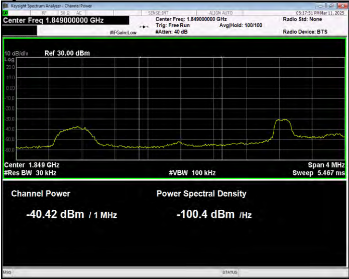
Band2 16QAM BW=3MHz Channel=18615 RB Size=15 Position=#0 Extended
