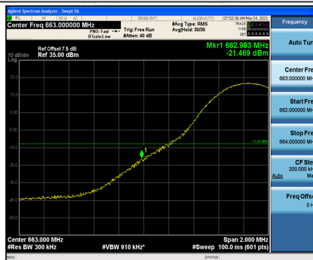
Band71-15MHz-16QAM-133197-1RB#74
