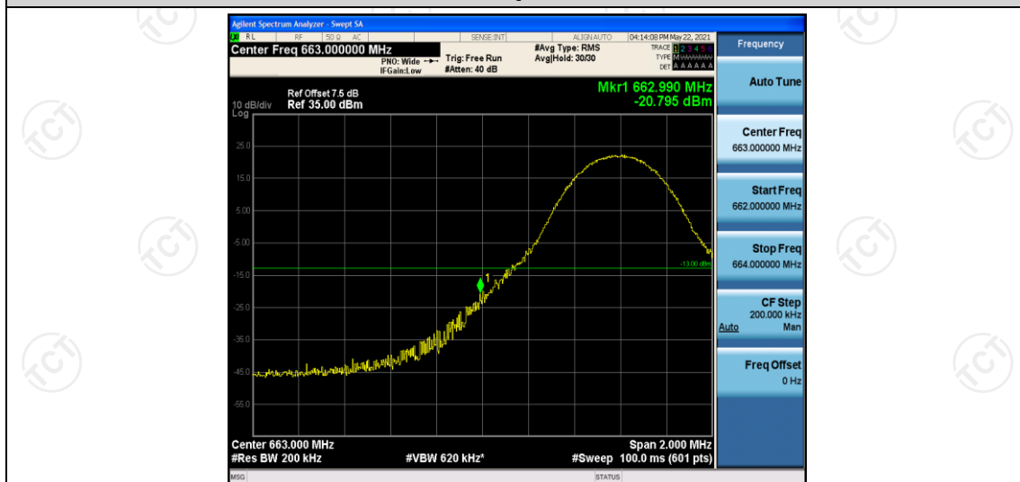
Band71-10MHz-16QAM-133172-1RB#49
