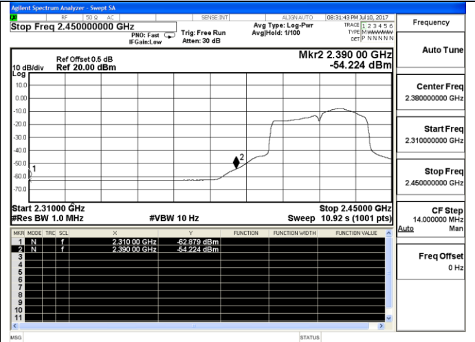
802.11n-HT40-Low channel(Average)
