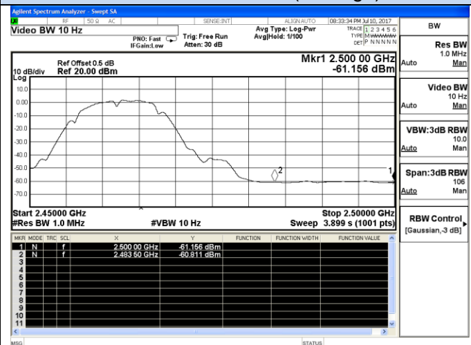
802.11b-High channel(Average)
