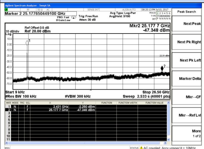
802.11n-HT40-Middle channel
