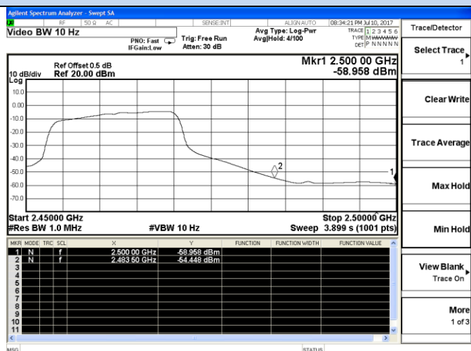
802.11g-High channel(Average)
