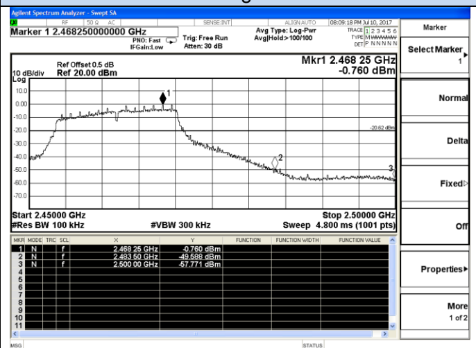
802.11g-High channel
