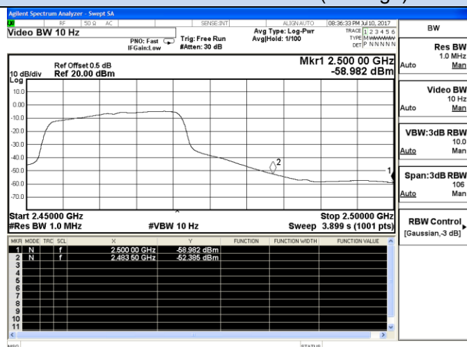
802.11n-HT20-High channel(Average)
