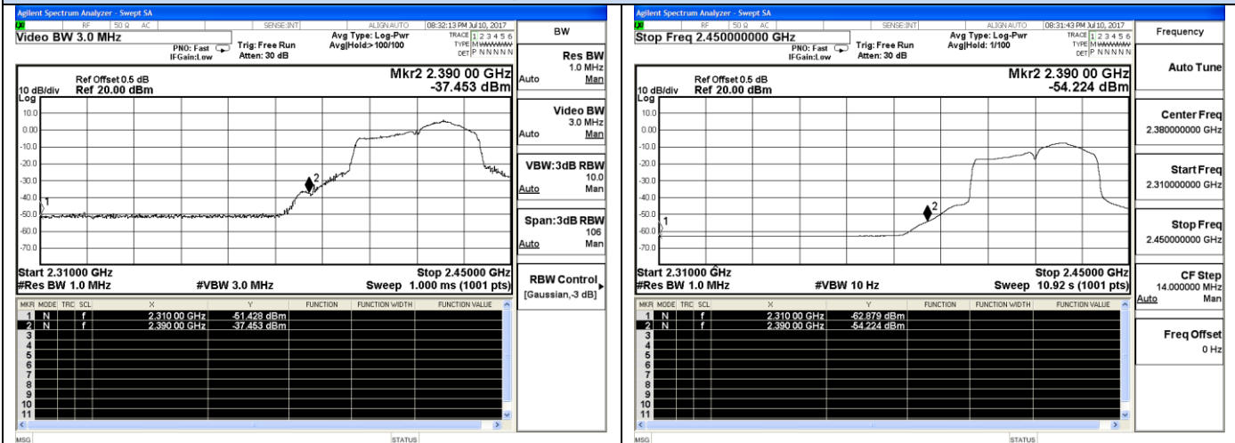
802.11n-HT40-Low channel(Peak)
