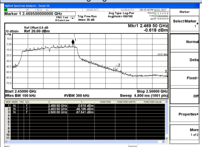
802.11n-HT20-High channel
