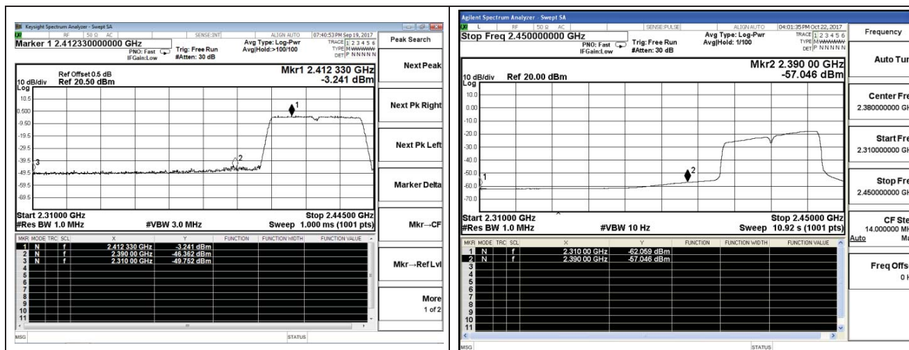
802.11n-HT40 Low channel(Peak)
