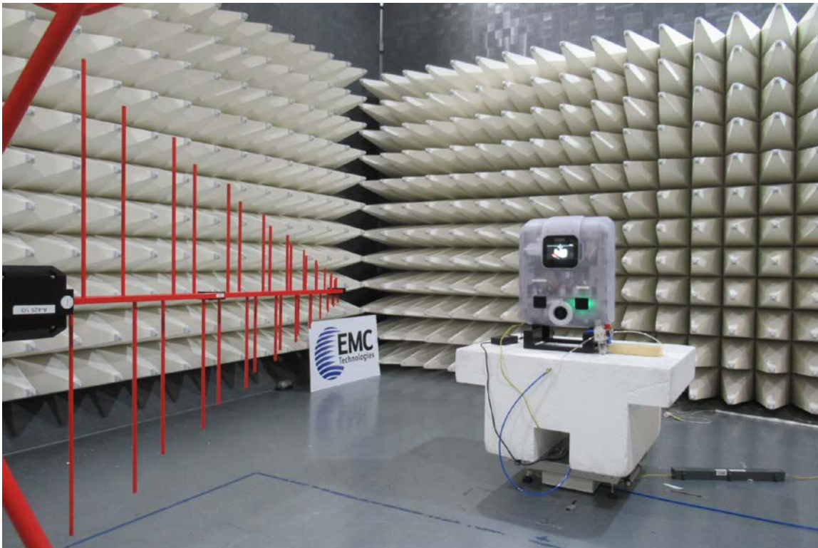
Above 30 MHz
