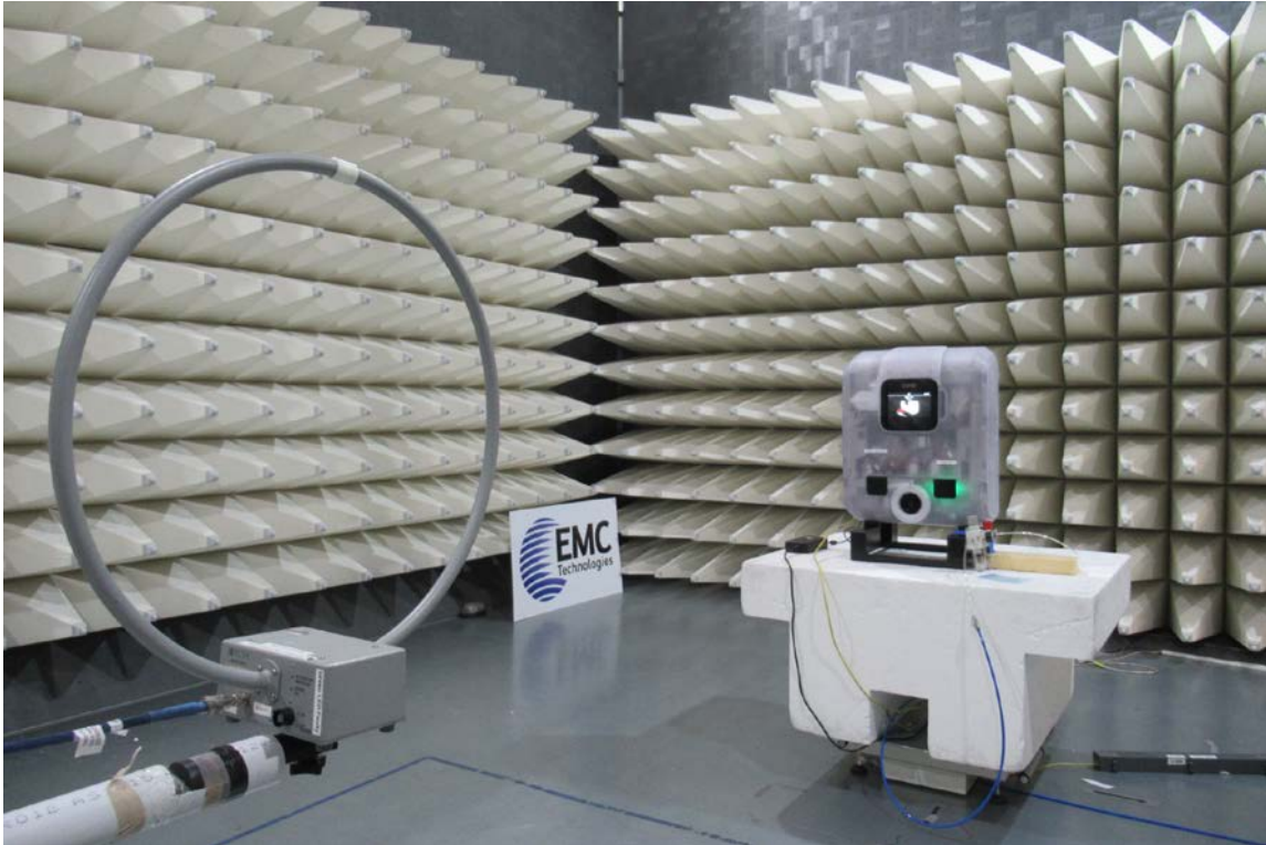
Below 30 MHz
