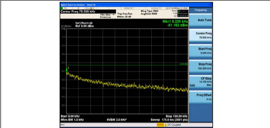
Band4_5MHz_QPSK_20375_1RB#0
