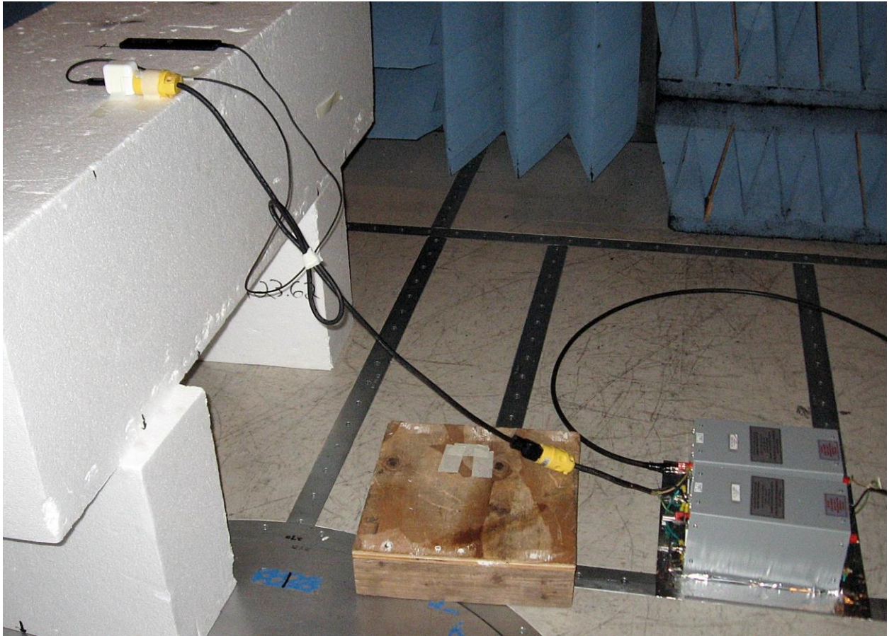
10. Tested conducted Emission during Charging.
