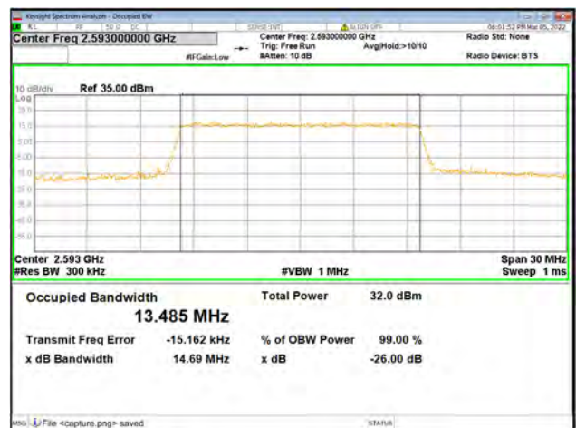
Band41 / 15MHz / Mid CH / 64QAM
