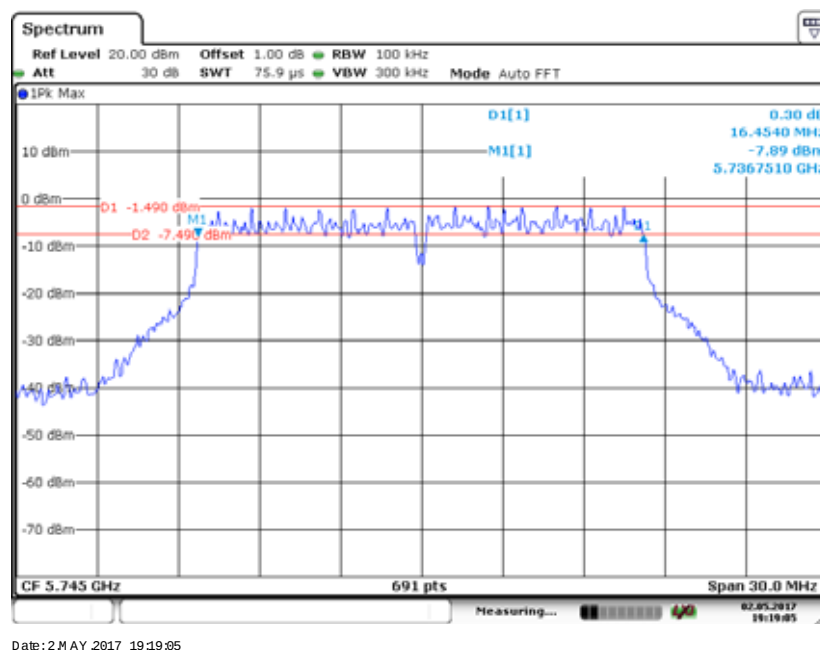
802.11a mode, Chain 0: 6 Bandwidth-5745MHz
