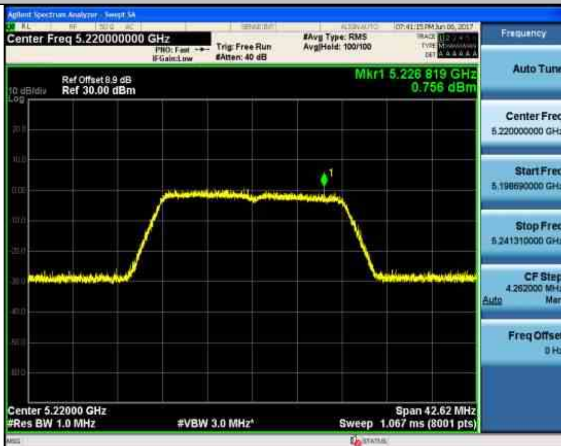
Maximum Conduct Output Power_TNVN_11AC20_5240_Ant1
