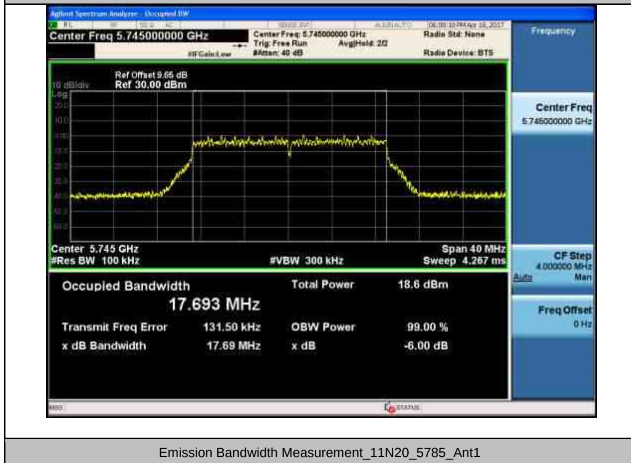
Emission Bandwidth Measurement_11N20_5745_Ant1
