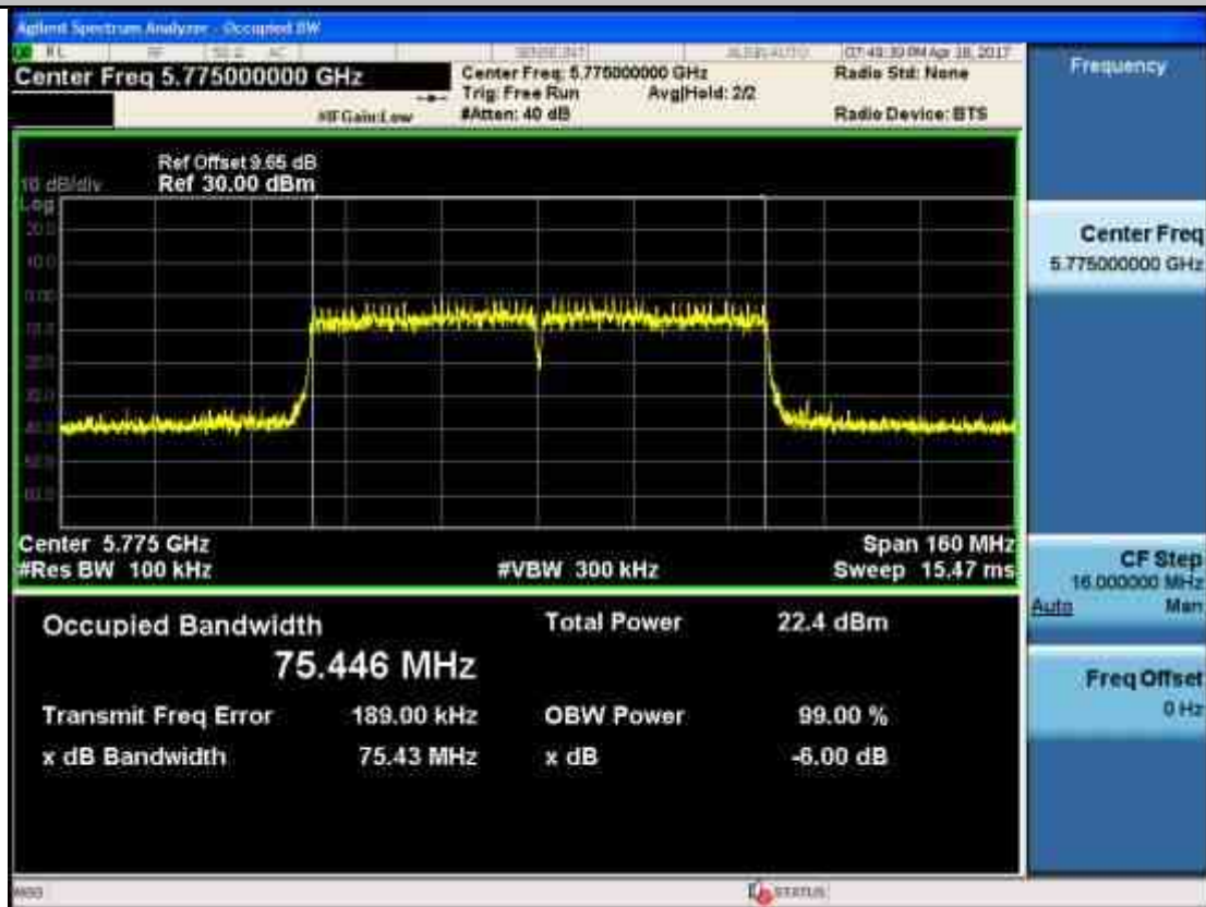
Emission Bandwidth Measurement_11AC80_5775_Ant1
