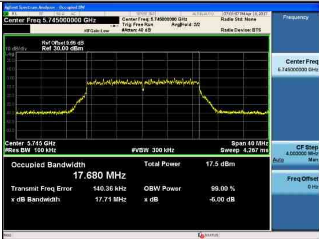
Emission Bandwidth Measurement_11AC20_5745_Ant1
