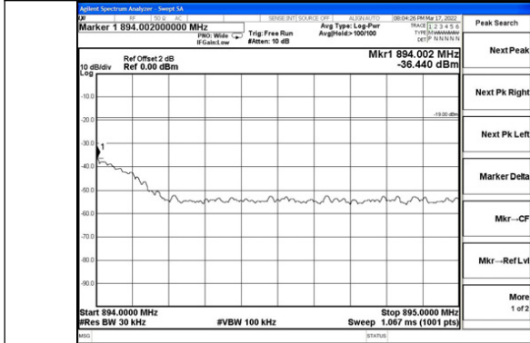
Cellular Band CDMA DL Right Side Pre AGC
