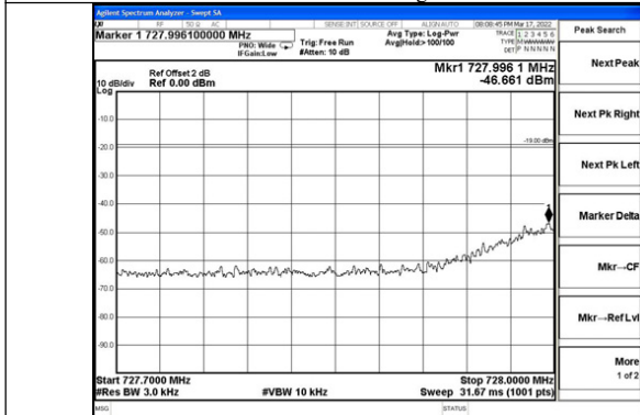
Lower 700MHz band CDMA DL Left Side Pre AGC
