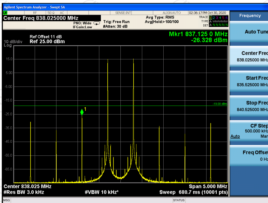
Band5 AGC +10dB, UL
