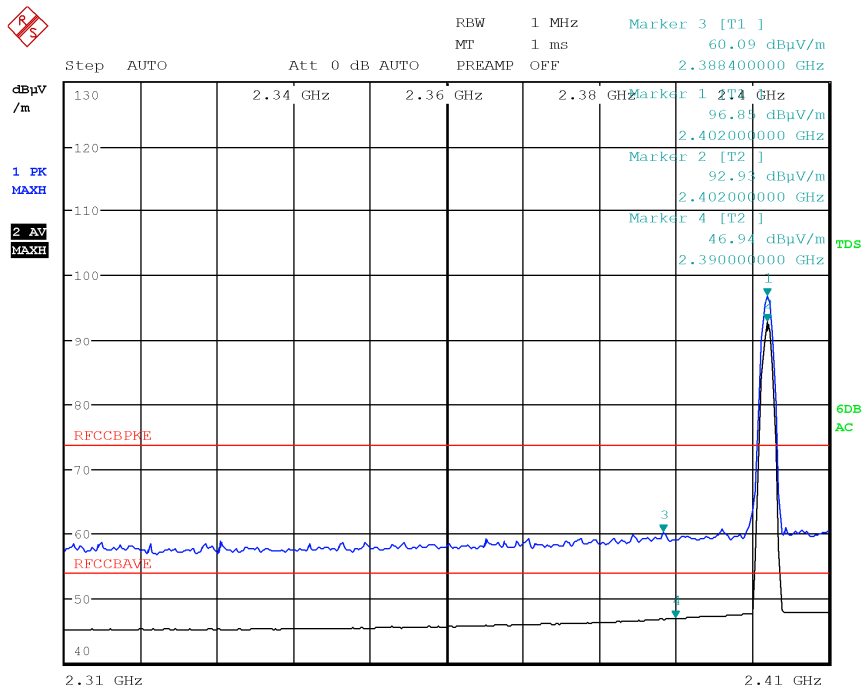
Figure 8.5-79: Bandedge, low channel BT worst case modulation 8DPSK with antenna in horizontal polarization
