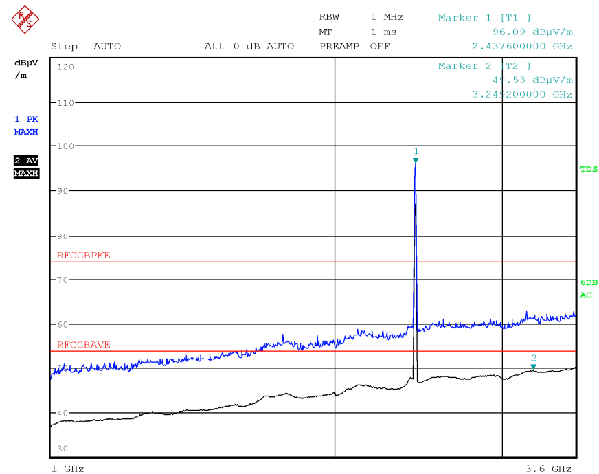
Figure 8.5-21: Radiated spurious emissions 1 to 3.6 GHz, Mid channel WiFi modulation 802.11b with antenna in horizontal polarization
