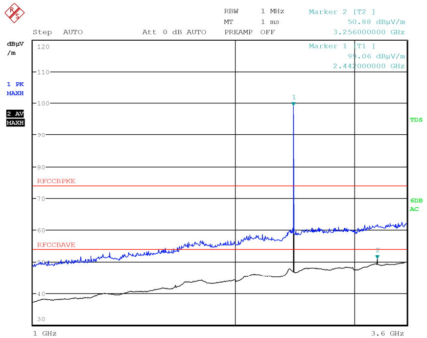
Figure 8.5-16: Radiated spurious emissions 1 to 3.6 GHz, Mid channel BLE with antenna in vertical polarization
