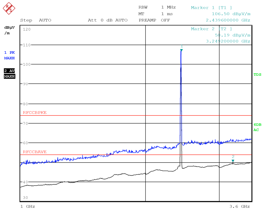
Figure 8.5-22: Radiated spurious emissions 1 to 3.6 GHz, Mid channel WiFi modulation 802.11b with antenna in vertical polarization
