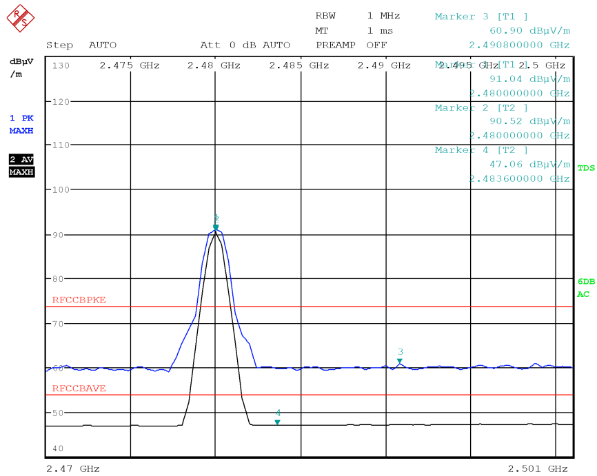
Figure 8.5-85: Bandedge, high channel BLE with antenna in horizontal polarization
