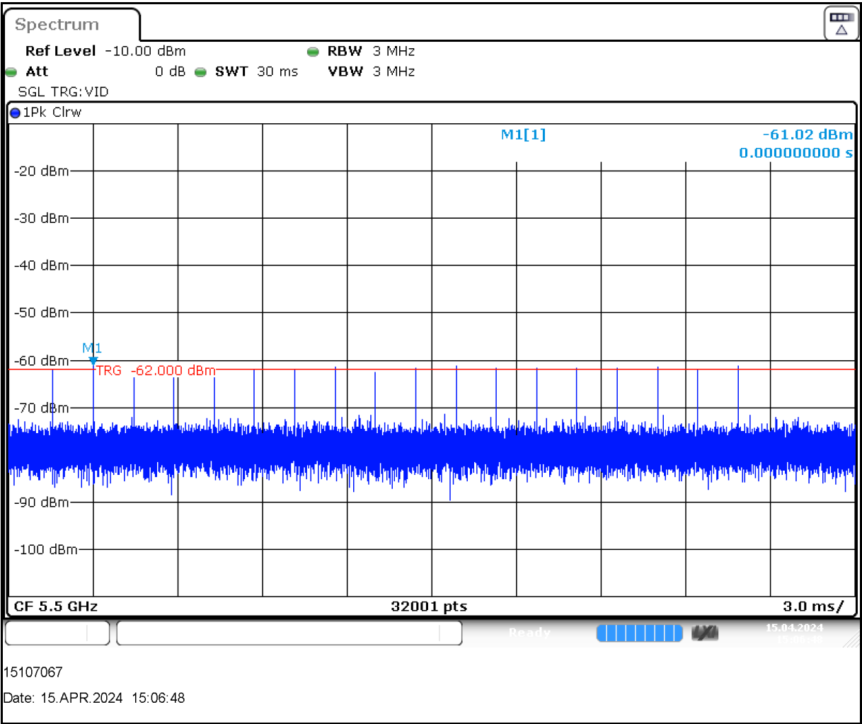
Radar Type 0 – full 18 pulse waveform
