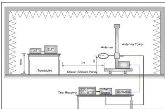
Figure 1. Below 30MHz
