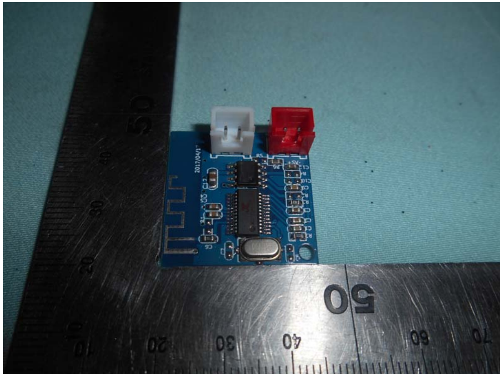
FIGURE 8 ELECTRIC HEATER (M/N: ND-36) BT BOARD (FRONT VIEW)
