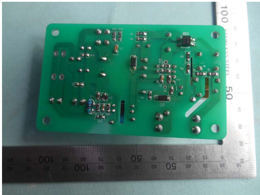
FIGURE 5 ELECTRIC HEATER (M/N: ND-36) POWER BOARD (BACK VIEW)
