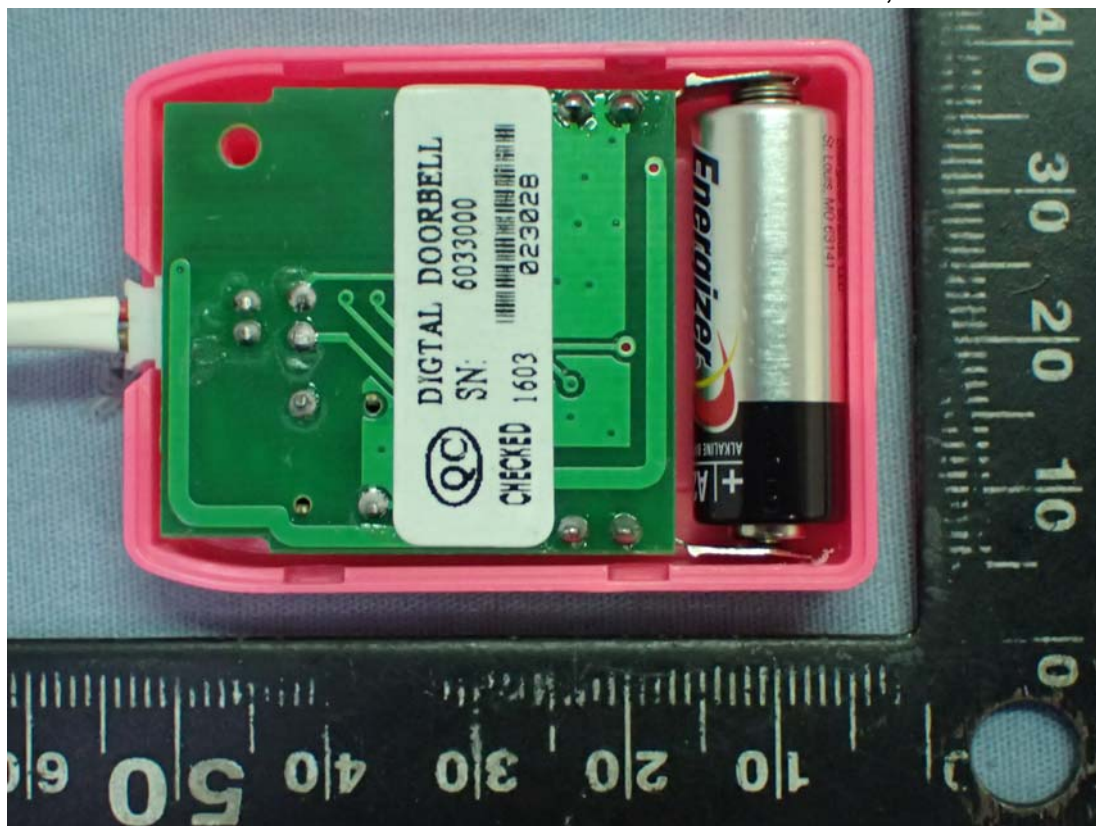
Figure 7 Transmitter, Internal View
