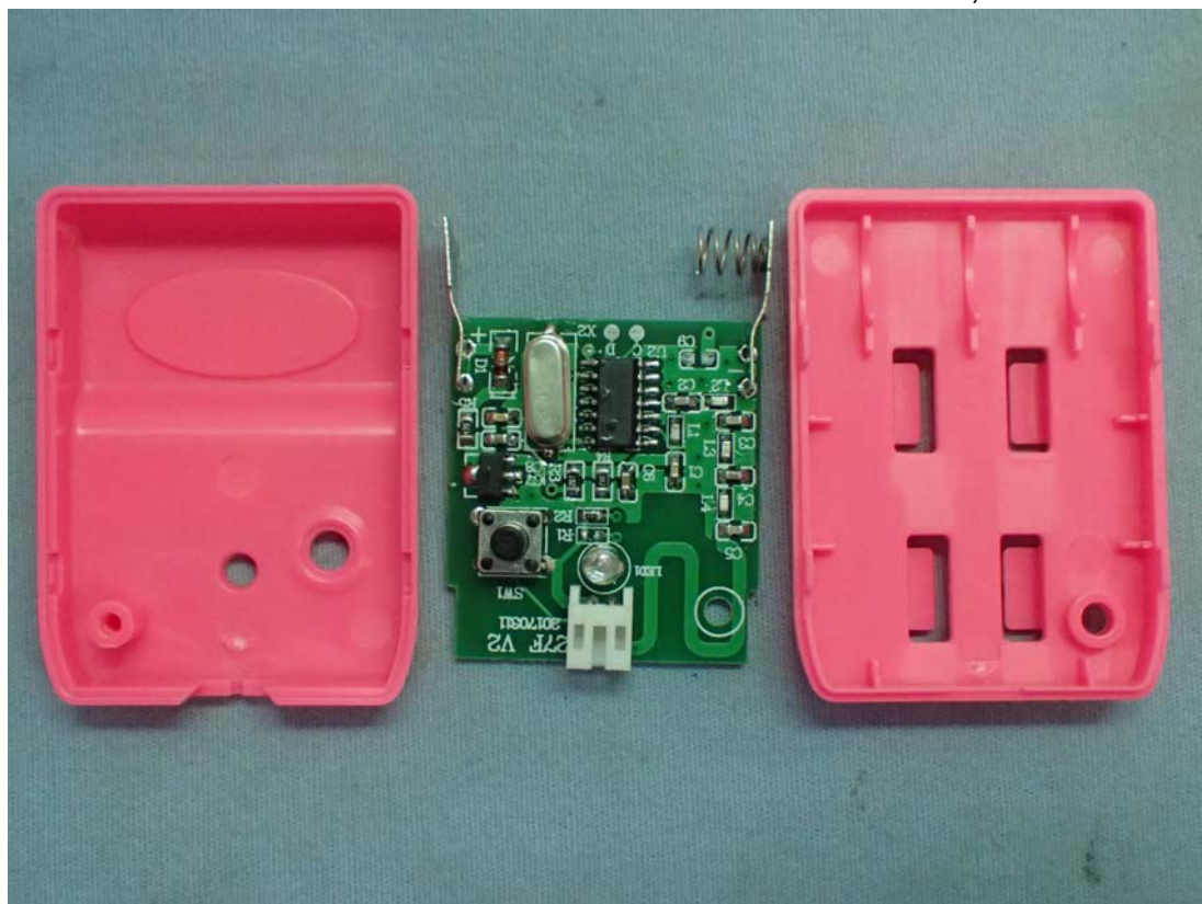
Figure 8 Transmitter, Internal View
