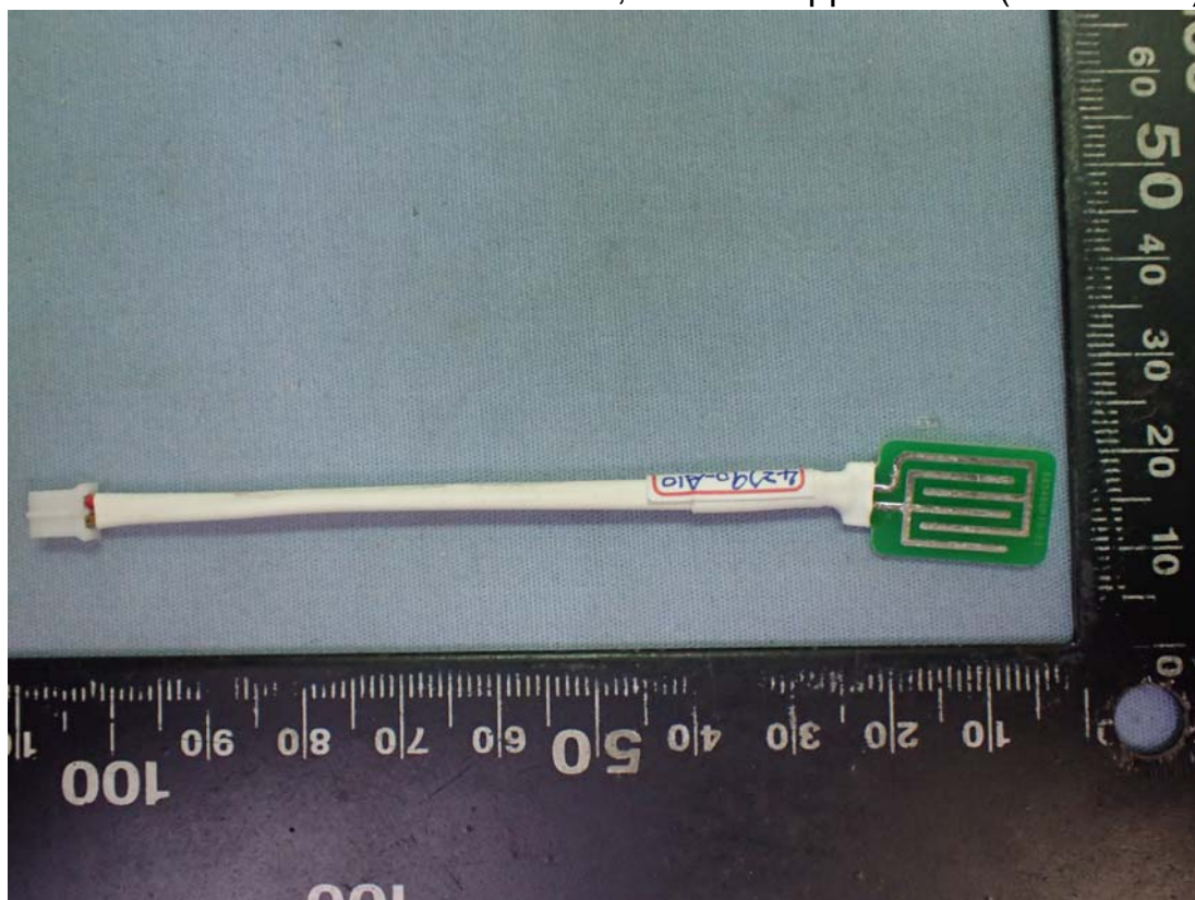
Figure 5 Sensor, General Appearance (Front View)
