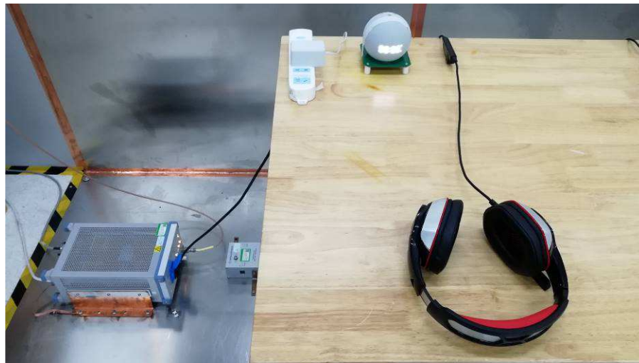
Photograph 3: Set-up photo for Conducted Emission on AC Mains
