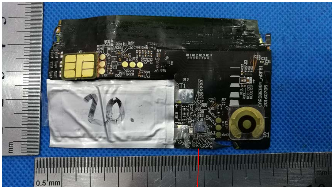
Antenna connected with component L3&C6
