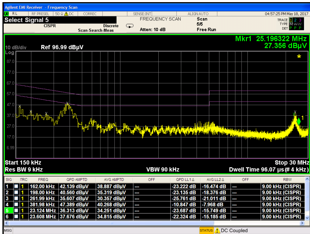
Plot 7-19. Line-Conducted Test Plot (N, RFID Antenna Terminated in 50Ω) (160143-915 (H318))
