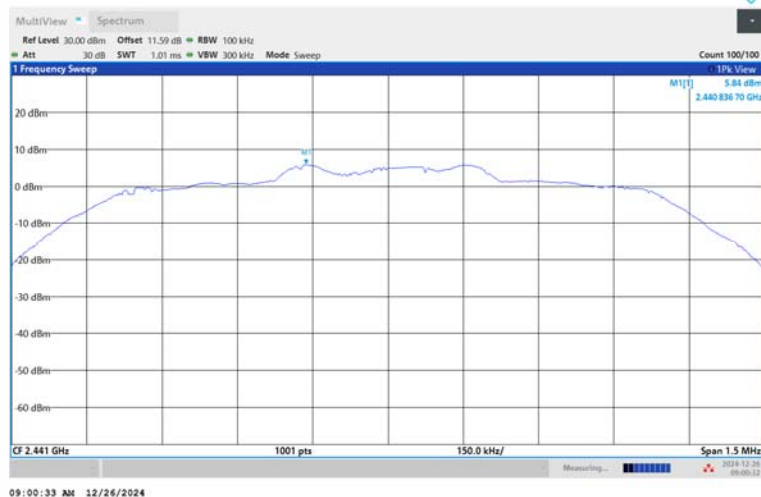
2DH5-Ant1-2441-PASS
