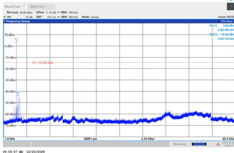
3DH5-Ant1-2402-1000~26500-PASS
