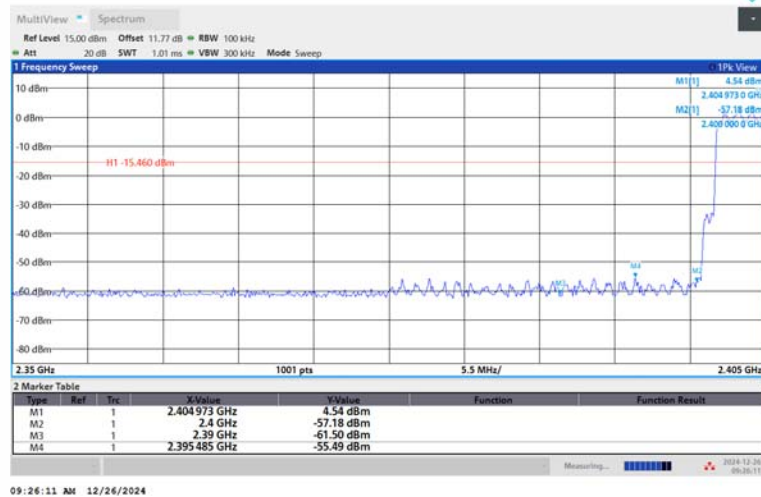
3DH5-Ant1-Hop_2402-PASS
