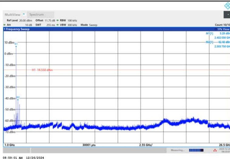
2DH5-Ant1-2402-1000~26500-PASS
