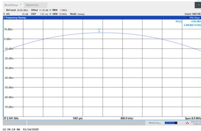
2DH5-Ant1-2441-PASS
