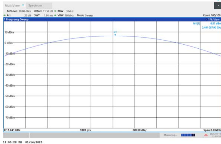
3DH5-Ant1-2441-PASS
