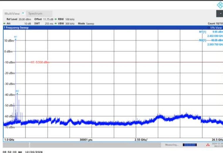
DH5-Ant1-2402-1000~26500-PASS
