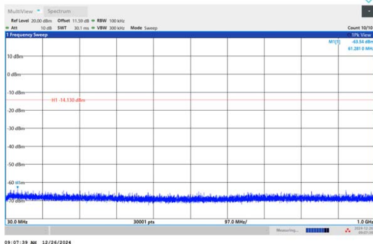
3DH5-Ant1-2441-30~1000-PASS
