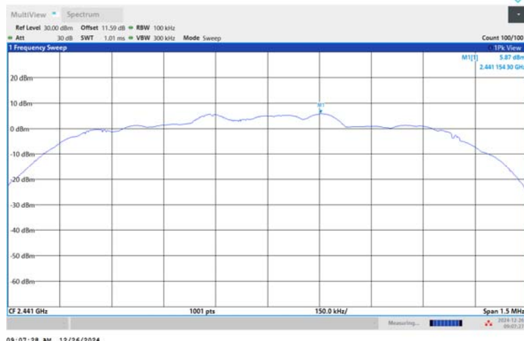
3DH5-Ant1-2441-PASS
