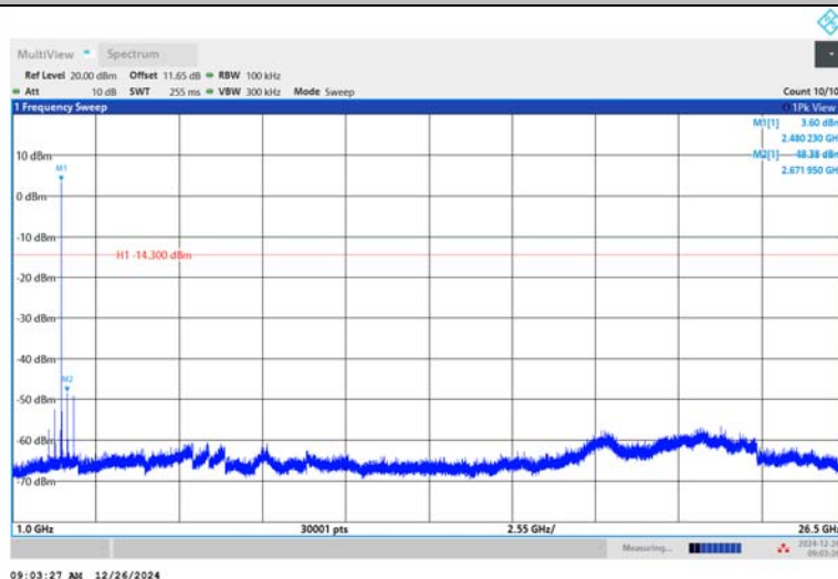
2DH5-Ant1-2480-1000~26500-PASS
