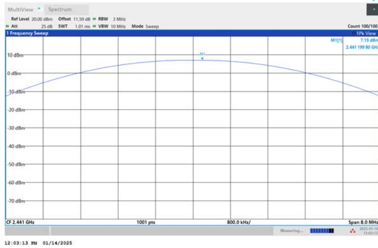
DH5-Ant1-2441-PASS
