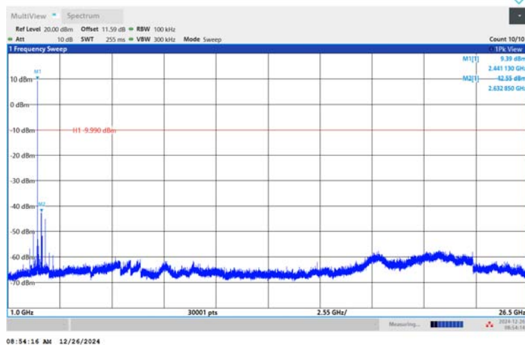
DH5-Ant1-2441-1000~26500-PASS
