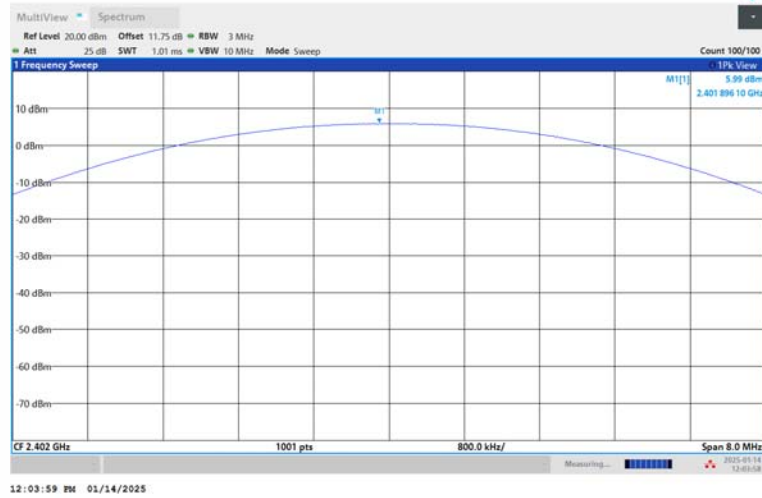
2DH5-Ant1-2402-PASS
