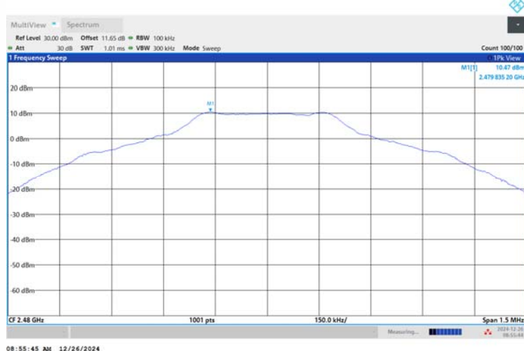
DH5-Ant1-2480-PASS
