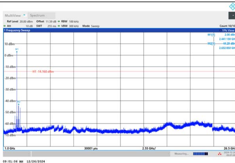
2DH5-Ant1-2441-1000~26500-PASS
