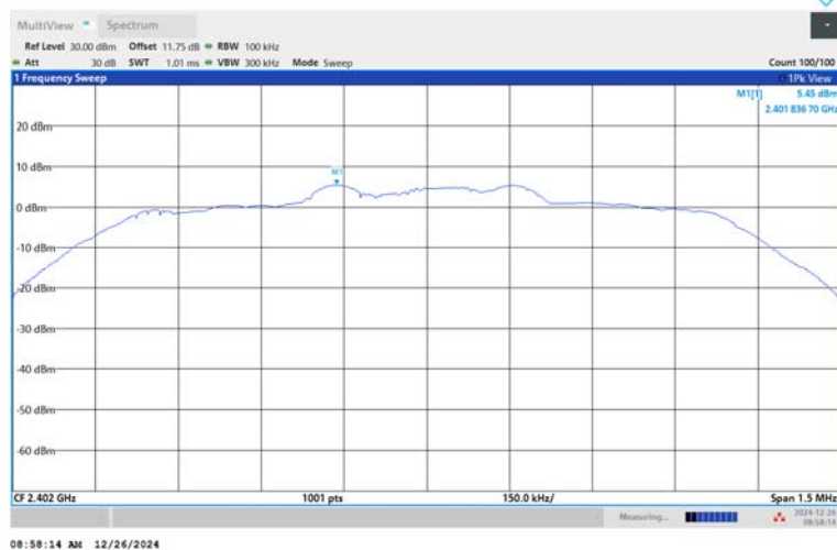
2DH5-Ant1-2402-PASS
