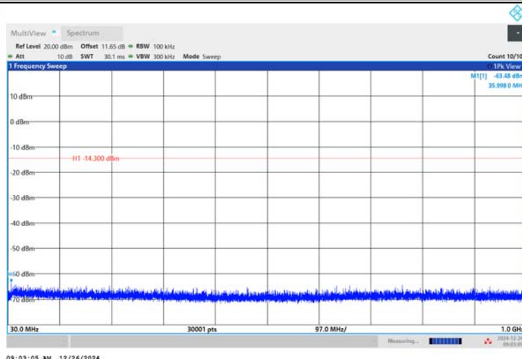
2DH5-Ant1-2480-30~1000-PASS
