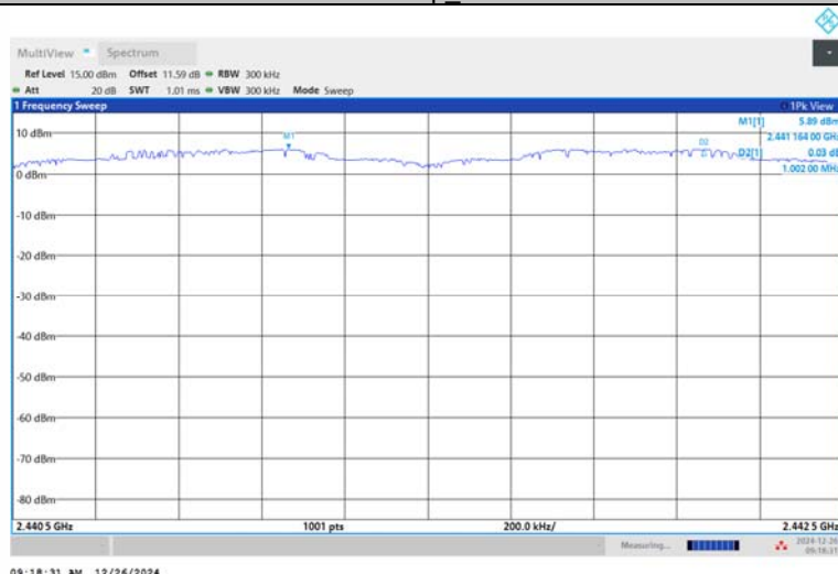
2DH5-Ant1-Hop_2441-PASS
