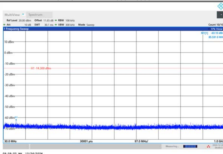
3DH5-Ant1-2480-30~1000-PASS
