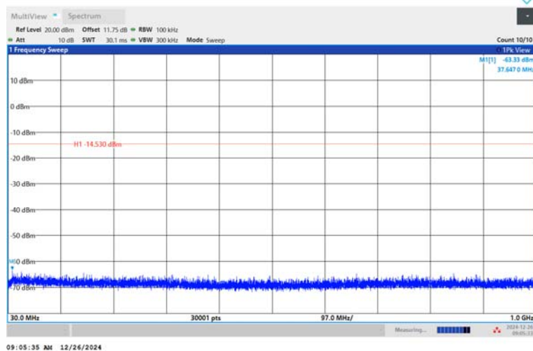
3DH5-Ant1-2402-30~1000-PASS
