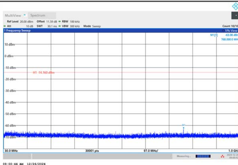
2DH5-Ant1-2441-30~1000-PASS
