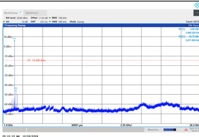
3DH5-Ant1-2480-1000~26500-PASS
