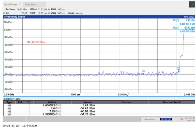
2DH5-Ant1-Hop_2402-PASS
