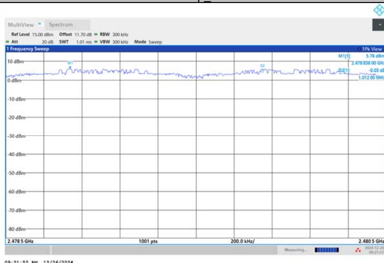
2DH5-Ant1-Hop_2480-PASS
