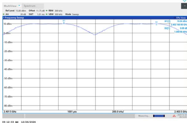
DH5-Ant1-Hop_2402-PASS
