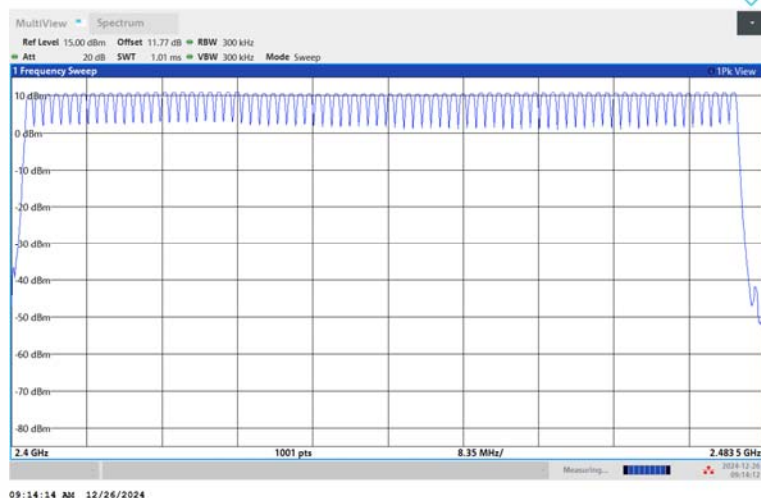
DH5-Ant1-Hop-PASS
