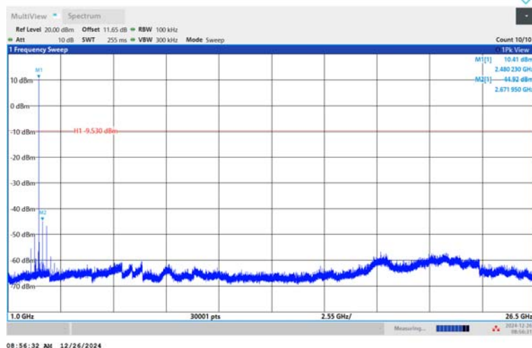
DH5-Ant1-2480-1000~26500-PASS
