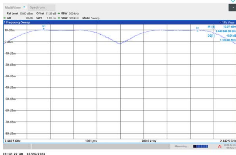
DH5-Ant1-Hop_2441-PASS
