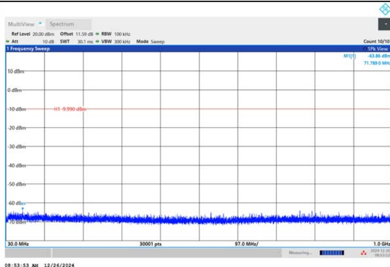
DH5-Ant1-2441-30~1000-PASS
