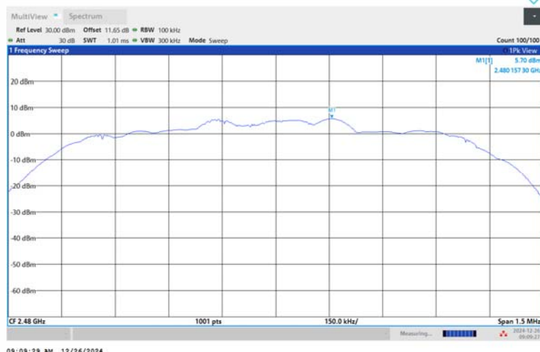
3DH5-Ant1-2480-PASS
