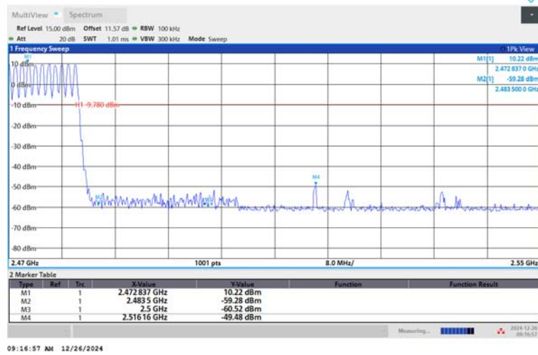
DH5-Ant1-Hop_2480-PASS
