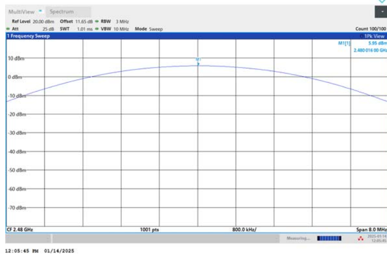
3DH5-Ant1-2480-PASS
