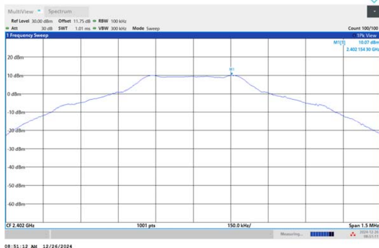
DH5-Ant1-2402-PASS
