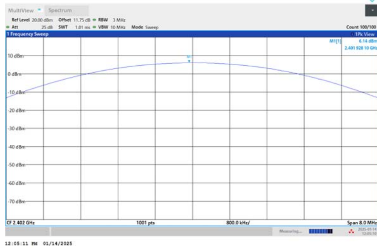
3DH5-Ant1-2402-PASS
