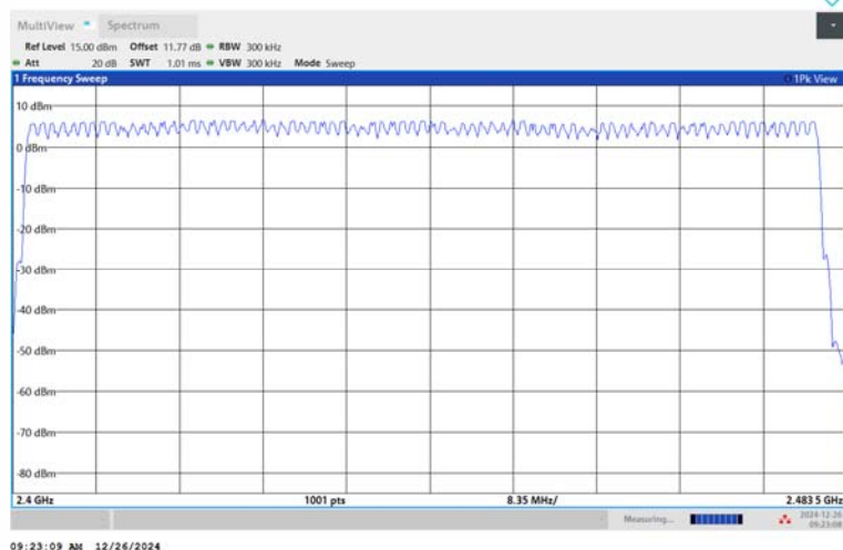
2DH5-Ant1-Hop-PASS
