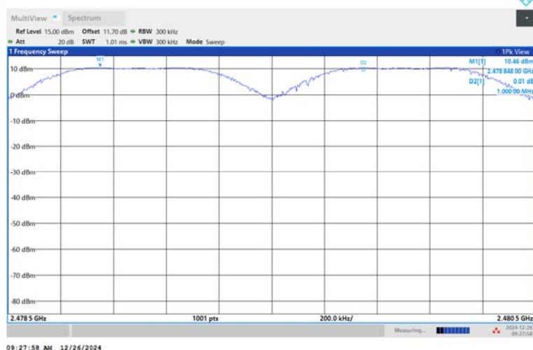
DH5-Ant1-Hop_2480-PASS
