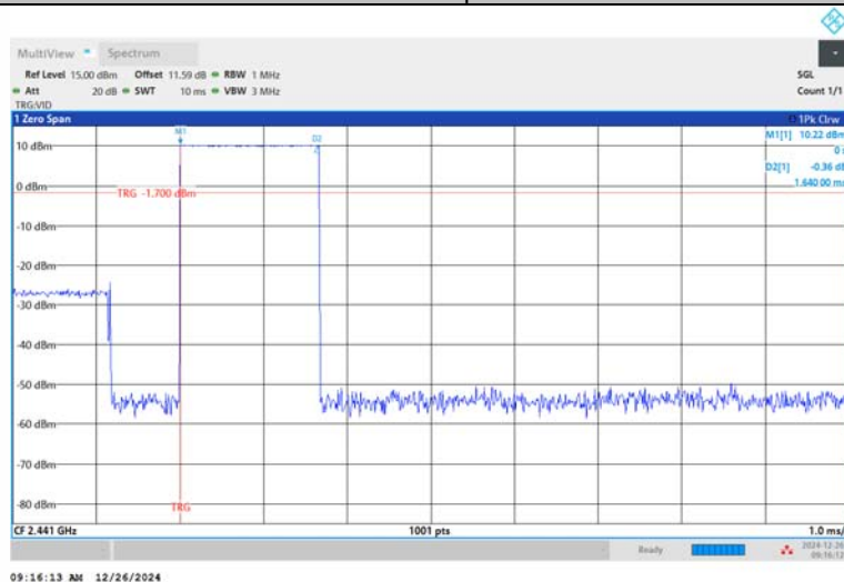
DH3-Ant1-Hop-PASS
