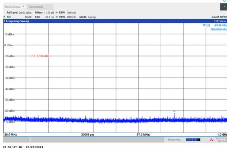
DH5-Ant1-2402-30~1000-PASS
