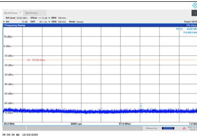
2DH5-Ant1-2402-30~1000-PASS
