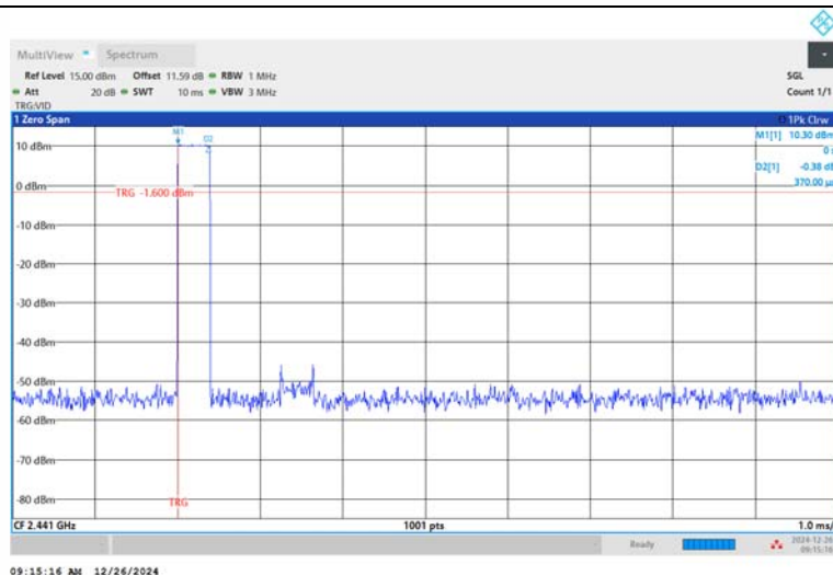
DH1-Ant1-Hop-PASS
