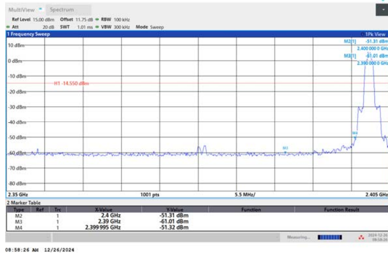
2DH5-Ant1-2402-PASS
