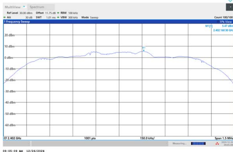
3DH5-Ant1-2402-PASS
