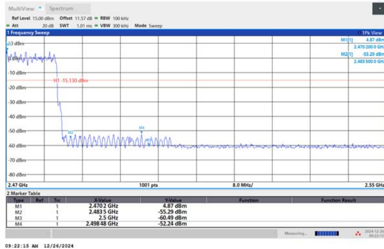
2DH5-Ant1-Hop_2480-PASS
