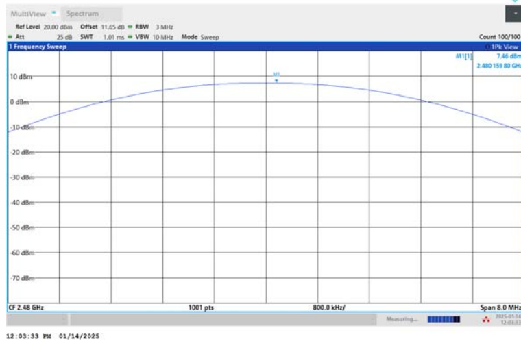
DH5-Ant1-2480-PASS
