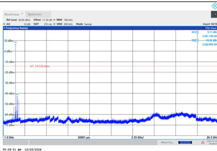
3DH5-Ant1-2441-1000~26500-PASS
