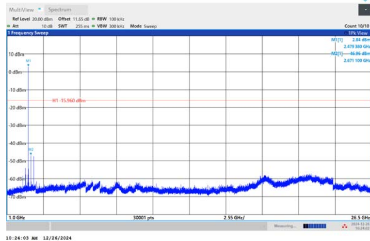
BLE_1M-Ant1-2480-1000~26500-PASS
