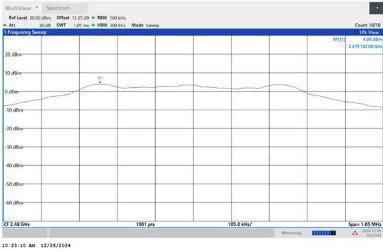
BLE_1M-Ant1-2480-PASS
