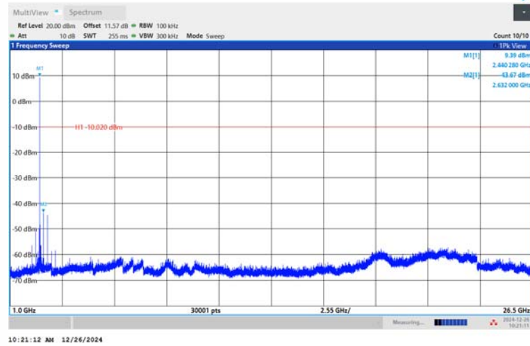
BLE_1M-Ant1-2440-1000~26500-PASS
