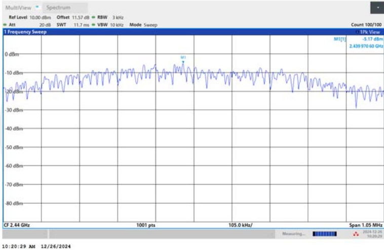
BLE_1M-Ant1-2440-PASS
