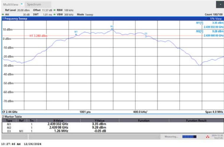
BLE_2M-Ant1-2440-PASS
