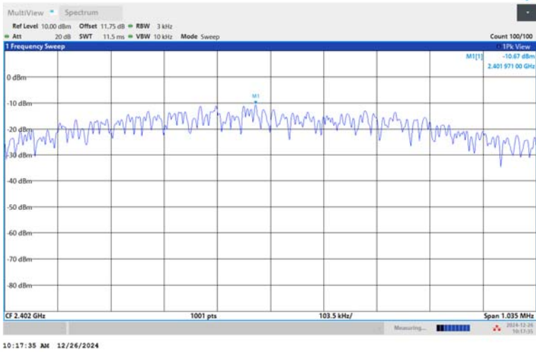
BLE_1M-Ant1-2402-PASS
