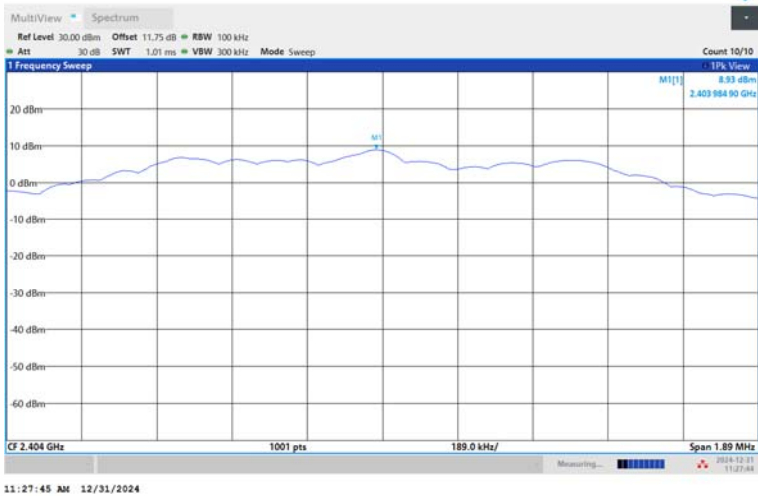
BLE_2M-Ant1-2404-PASS
