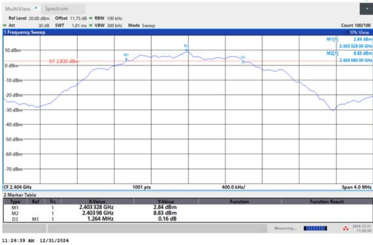
BLE_2M-Ant1-2404-PASS
