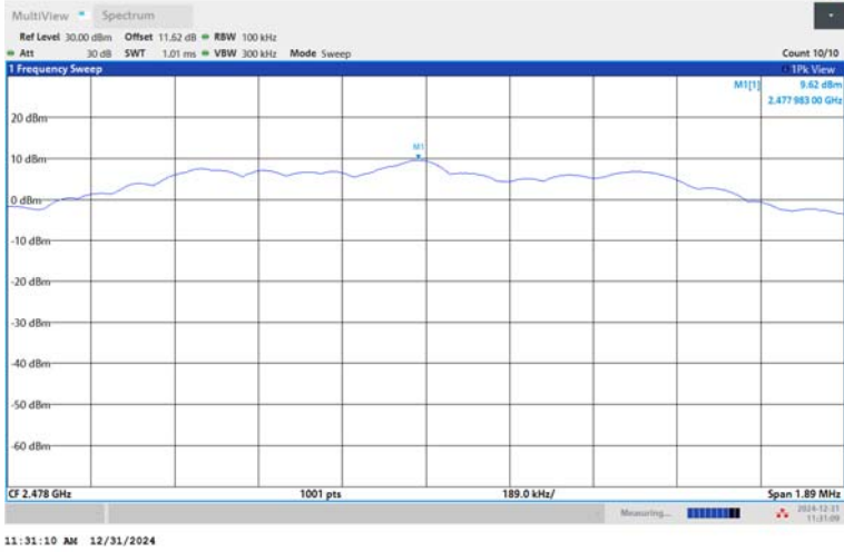
BLE_2M-Ant1-2478-PASS
