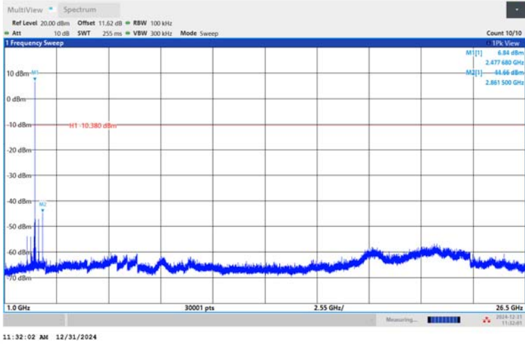
BLE_2M-Ant1-2478-1000~26500-PASS
