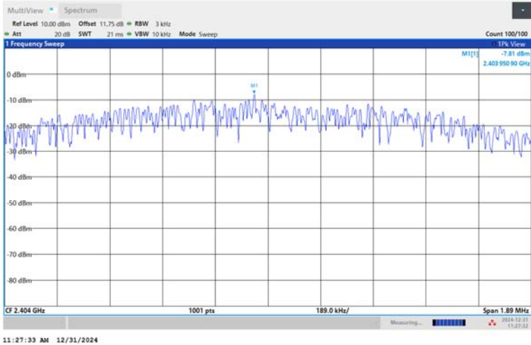
BLE_2M-Ant1-2404-PASS
