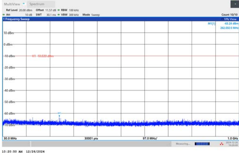
BLE_1M-Ant1-2440-30~1000-PASS
