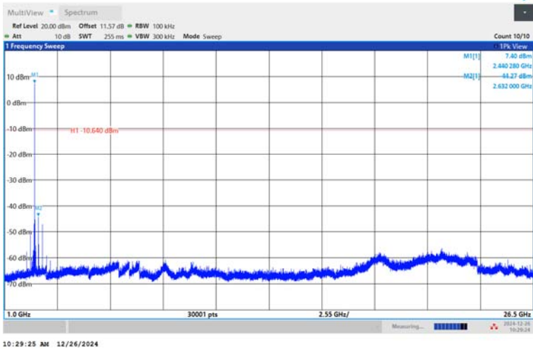
BLE_2M-Ant1-2440-1000~26500-PASS
