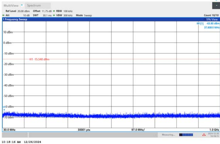
BLE_1M-Ant1-2402-30~1000-PASS
