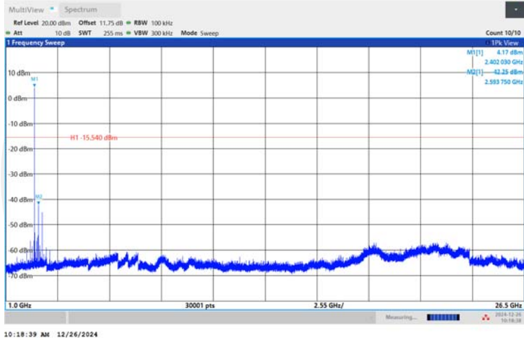
BLE_1M-Ant1-2402-1000~26500-PASS
