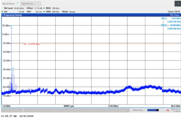
BLE_2M-Ant1-2404-1000~26500-PASS
