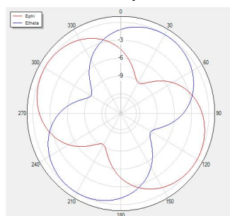
H Theta=0 freq=2450MHz
