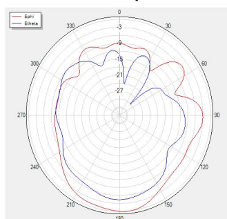
H Theta=90 freq=2450MHz
