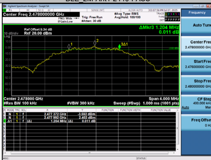
BLE_2M-Ant1-2478-PASS
