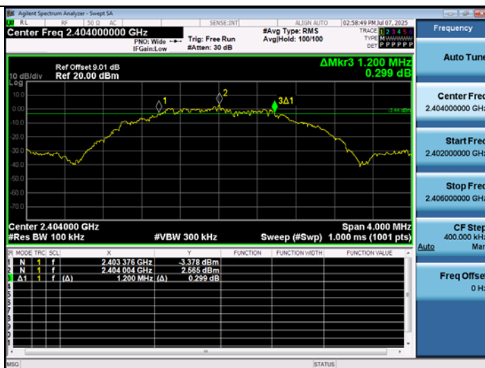
BLE_2M-Ant1-2404-PASS
