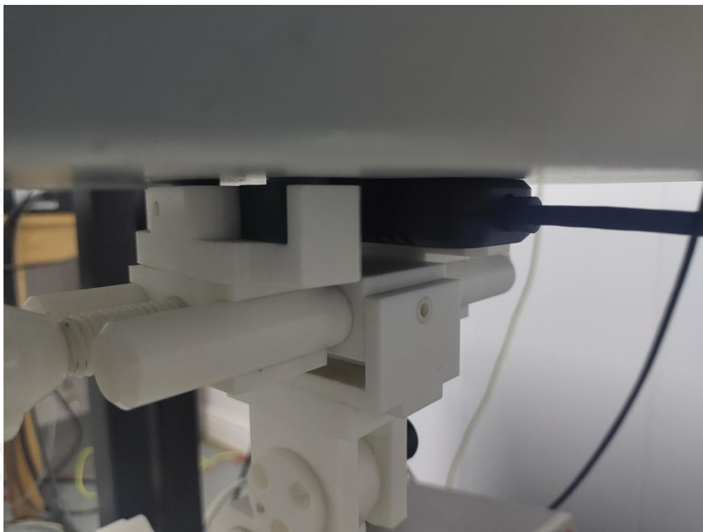
0mm body Horizontal-Up Side Setup Photo – Test Position 2
