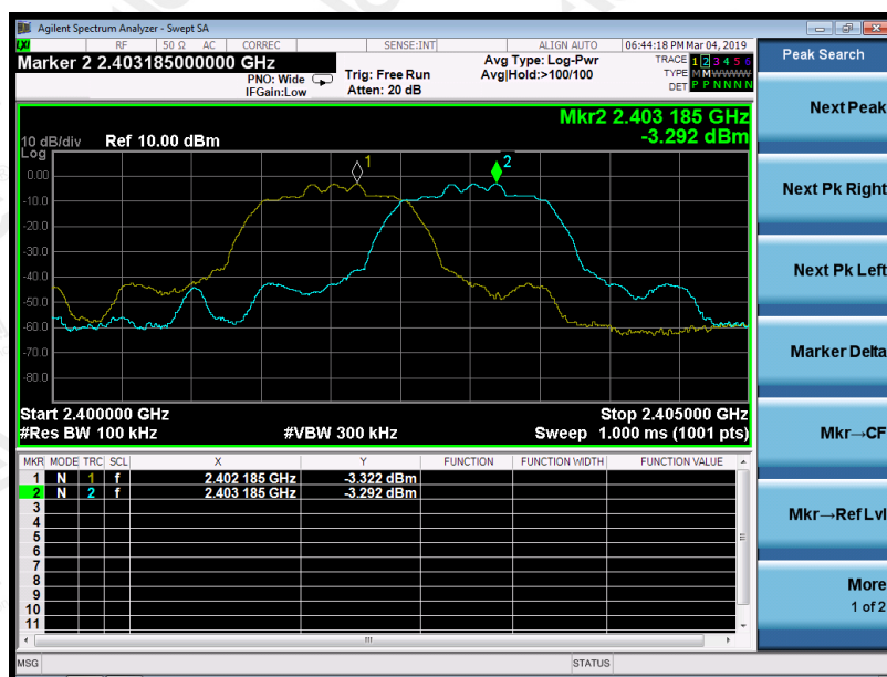
TEST PLOT FOR FREQUENCY SEPARATION ( 2Mbps )
