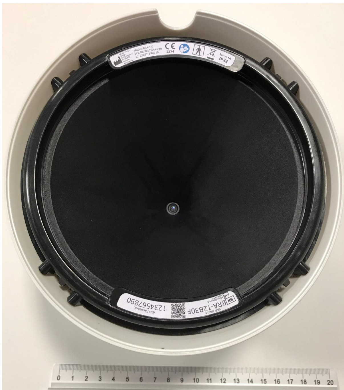
Fig. 2 – Bottom view of BRA-1.0
