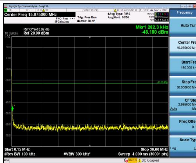
Band4-1413-4-0.15~30MHz
