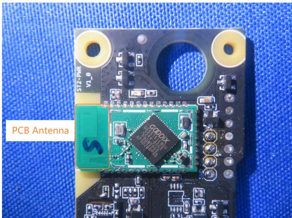
(12) EUT Photo (GR5515 Bluetooth Chip)
