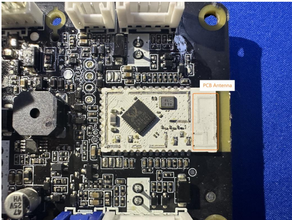
(6) EUT Photo (MHCB05P-B Bluetooth Chip)
