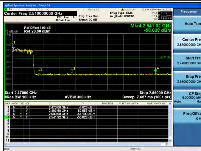
3DH5_Ant1_High_Hop_2480
