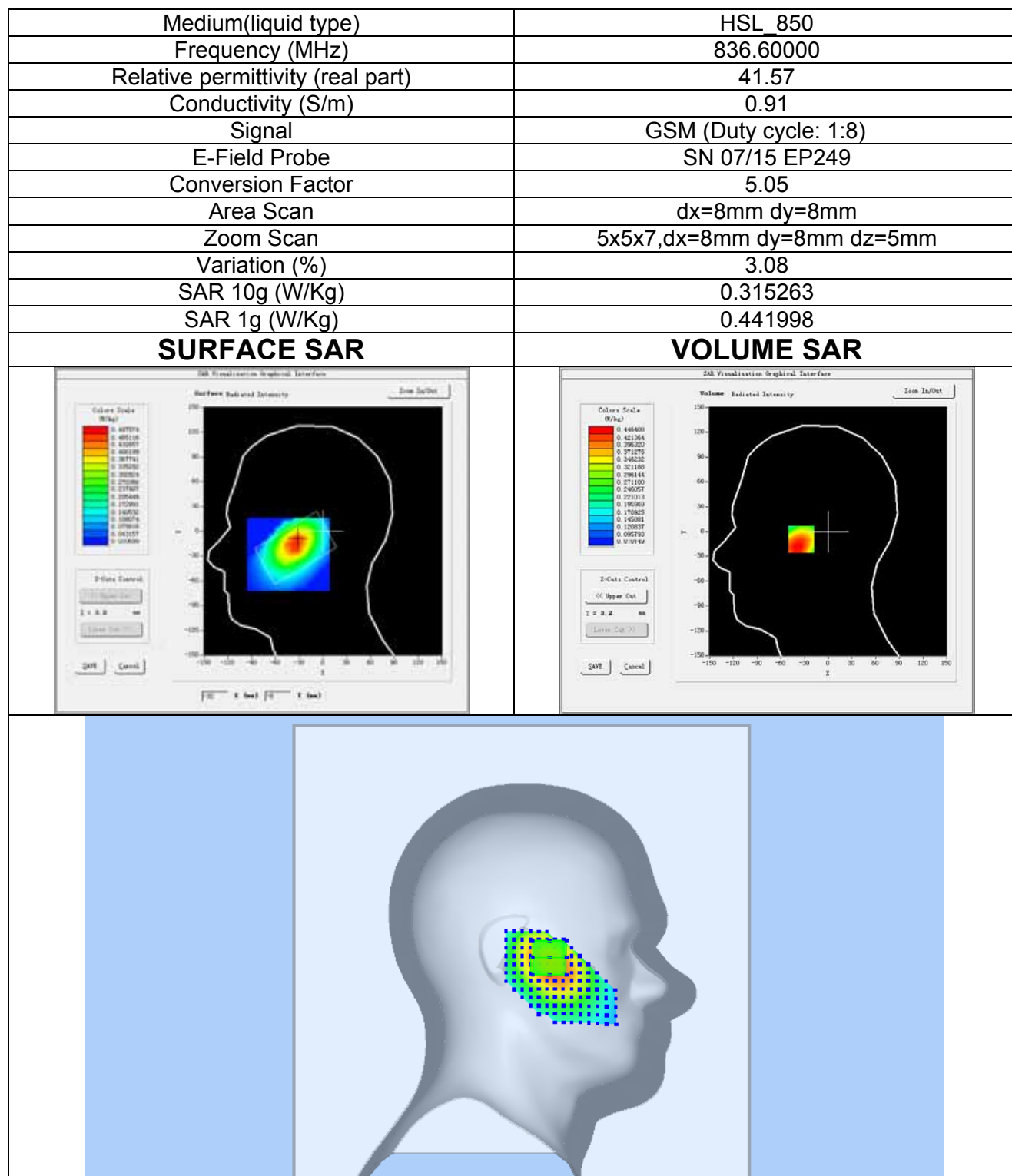
Plot 4: GSM850MHz, Middle channel (Left Head , Tilt) Product Description: Mobile Phone Test Date: Apr 17, 2017
