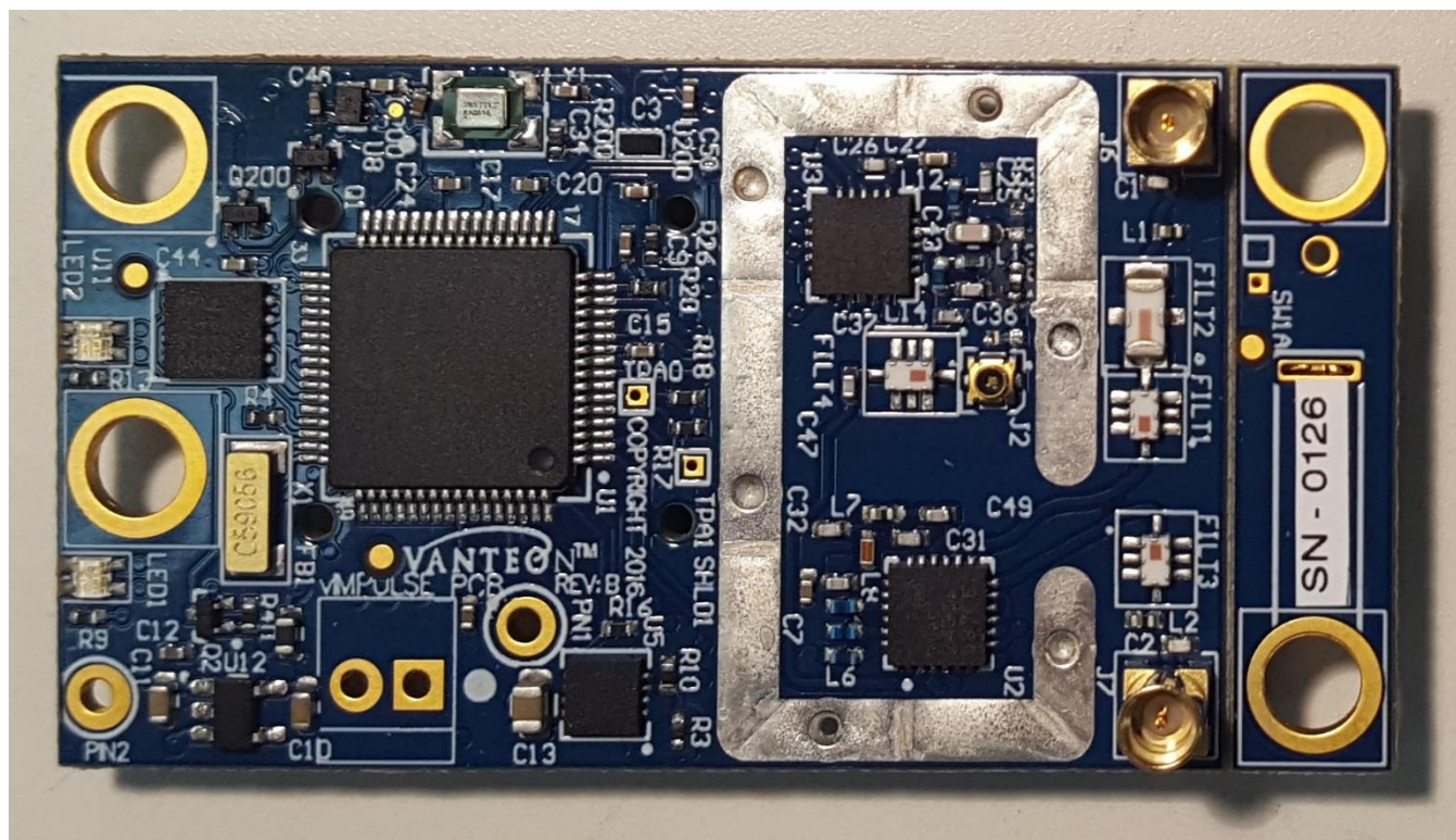
Figure 1: Top View
