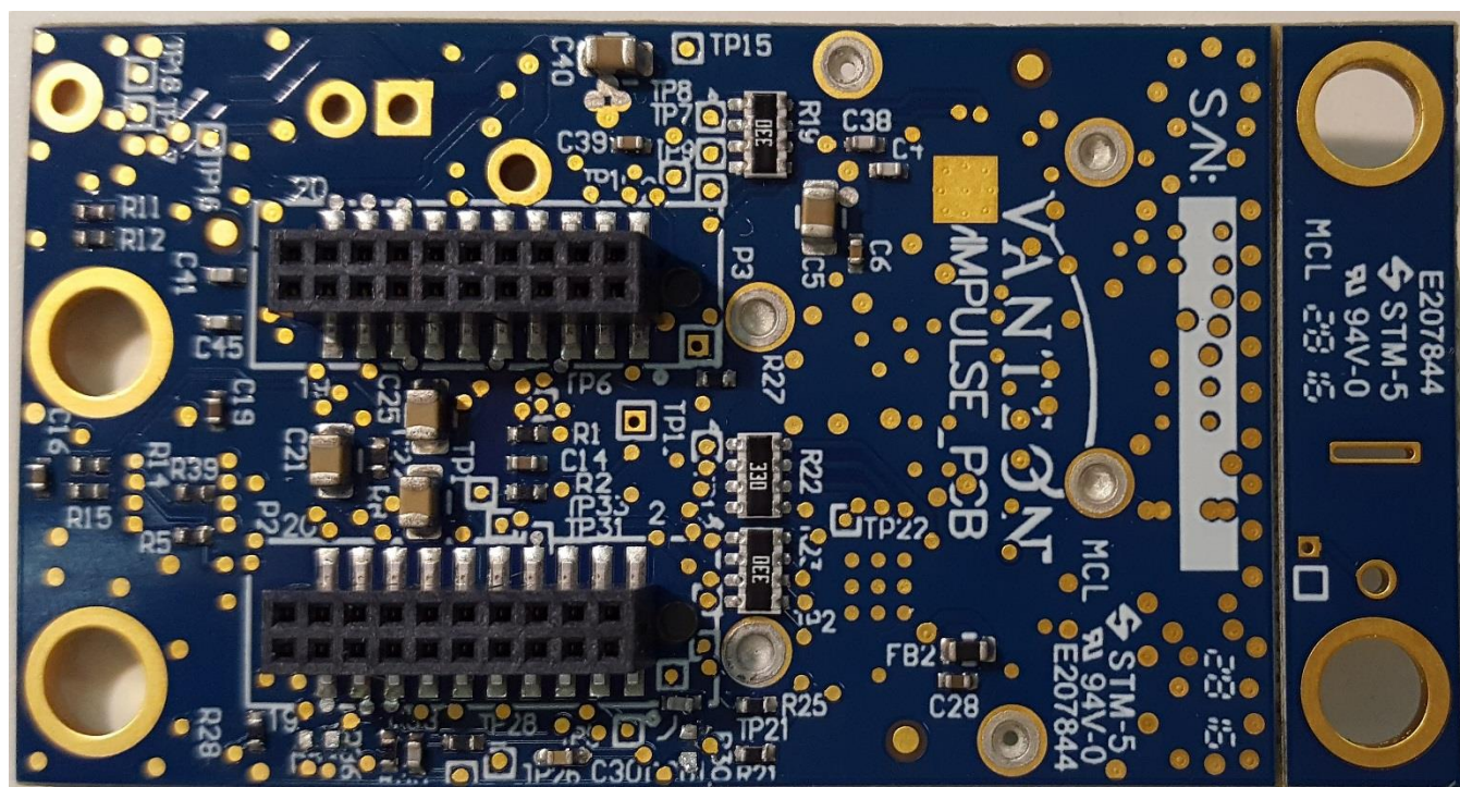
Figure 2: Bottom View
