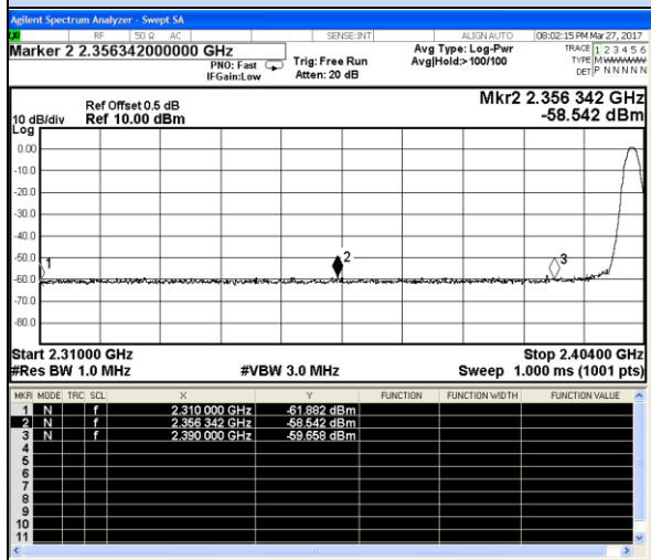
Channel 0 / 2402 MHz – Non-Hopping – Peak
