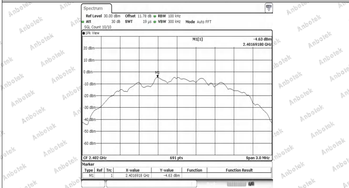
BLE_2M-Ant1-2402-0~Reference-PASS
