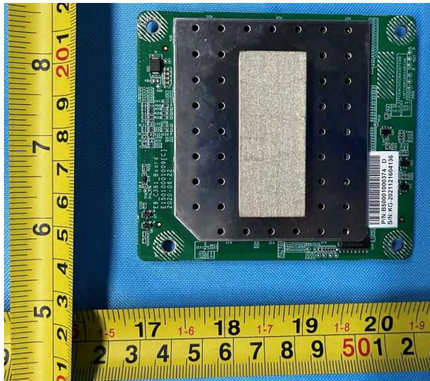
Internal View of EUT-14
