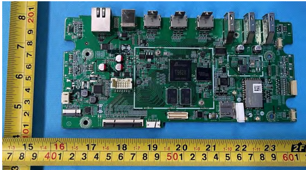
Internal View of EUT-10
