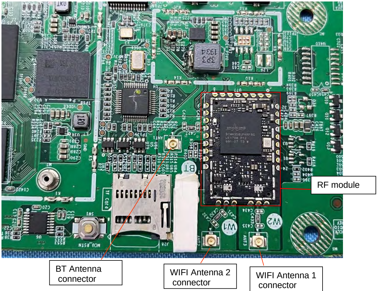
Detail view of RF module
