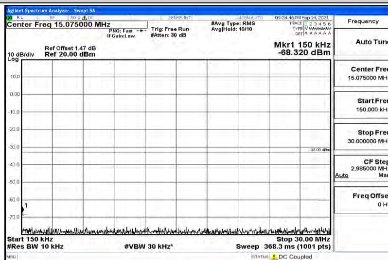
Band66-15MHz-QPSK-132047-Range3:30~1000MHz
