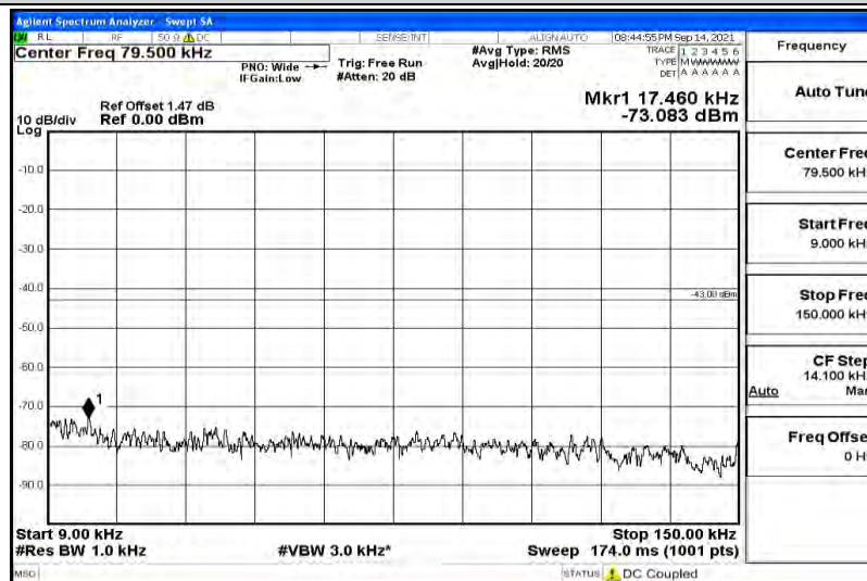
Band66-5MHz-16QAM-131997-Range2:0.15~30MHz
