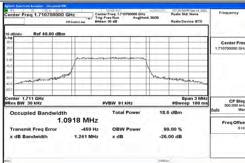
Band66-1.4MHz-16QAM-132322
