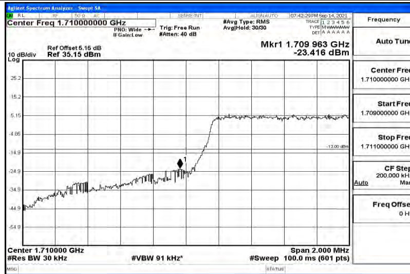
Band66-1.4MHz-QPSK-132665
