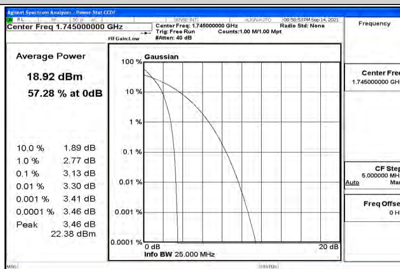
Band66-5MHz-QPSK-132647
