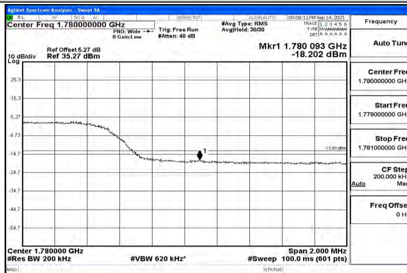
Band66-15MHz-QPSK-132047
