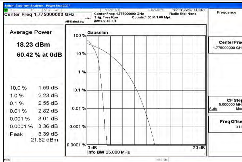
Band66-10MHz-16QAM-132022
