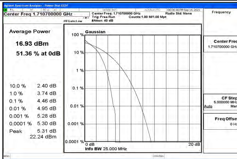
Band66-1.4MHz-QPSK-132322
