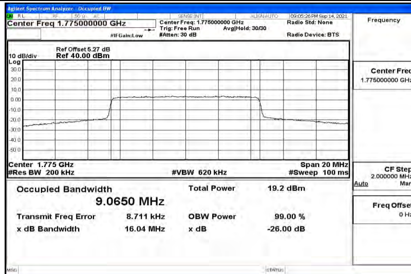
Band66-10MHz-16QAM-132022
