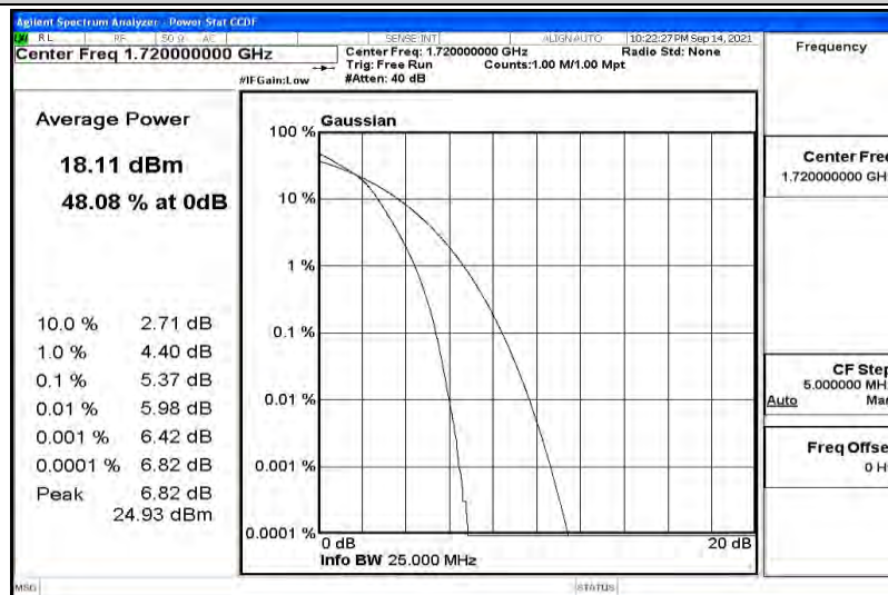
Band66-20MHz-16QAM-132322
