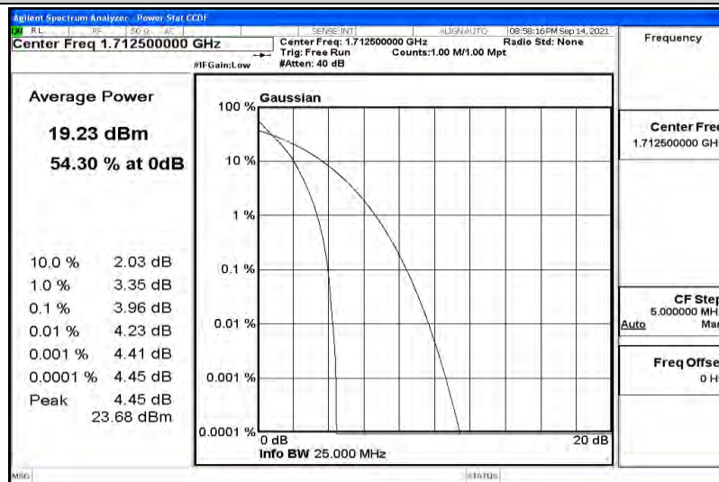
Band66-5MHz-QPSK-132322
