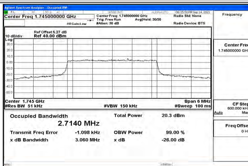
Band66-3MHz-16QAM-132657
