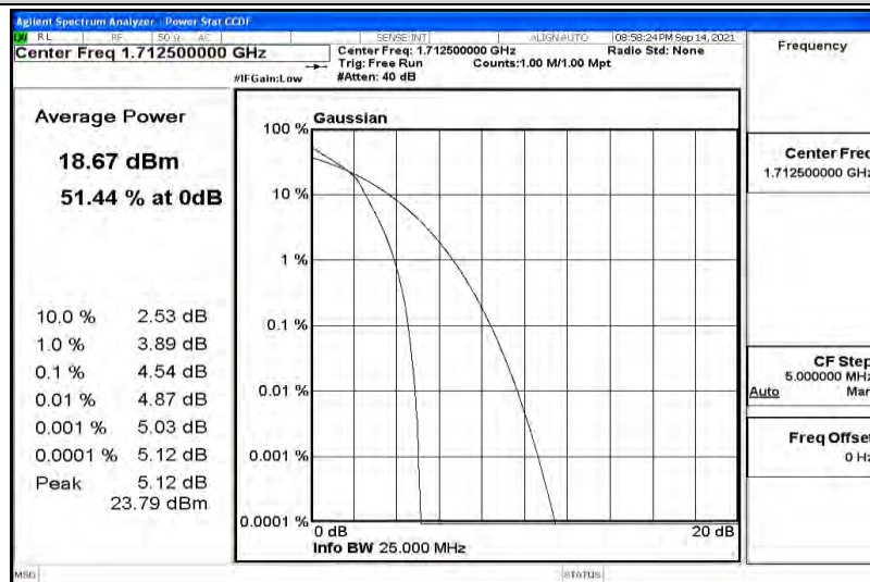
Band66-5MHz-16QAM-132322
