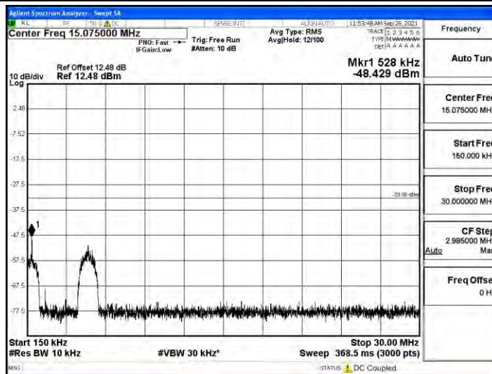
(Channel Bandwidth: 1.4 MHz)_LCH_QPSK
