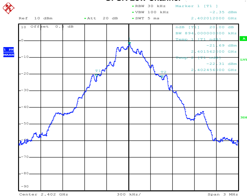
Test plots GFSK Low Channel
