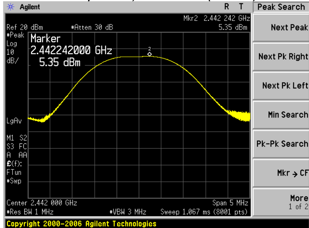
Maximum Peak Output Power, Middle Channel (2442 MHz)
