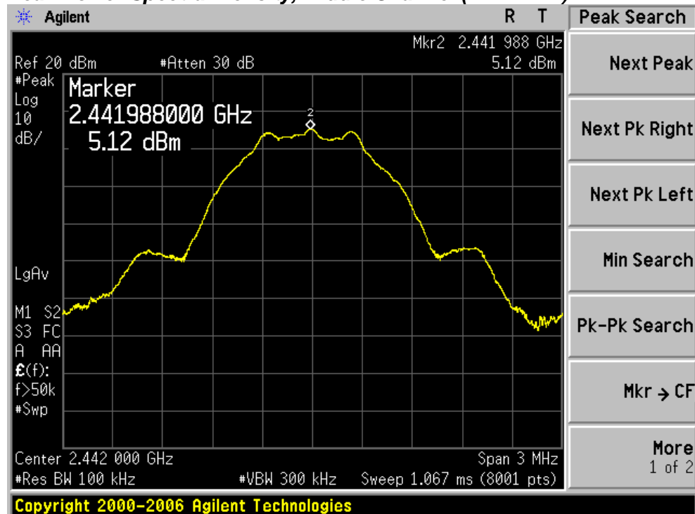
Peak Power Spectral Density, Middle Channel (2442 MHz)
