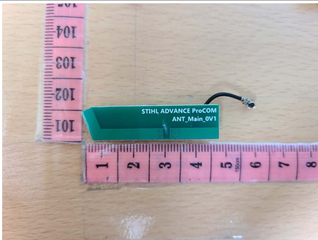
Mesh Antenna1
