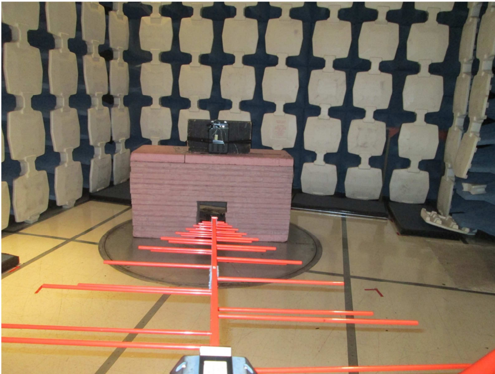
Radiated Spurious Emissions (30MHz - 1GHz)
