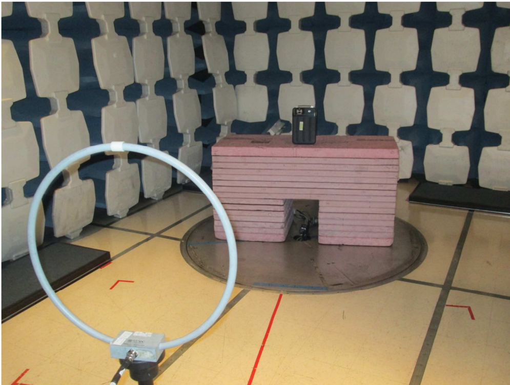
Fundamental and Radiated Spurious Emissions (9kHz - 1MHz)
