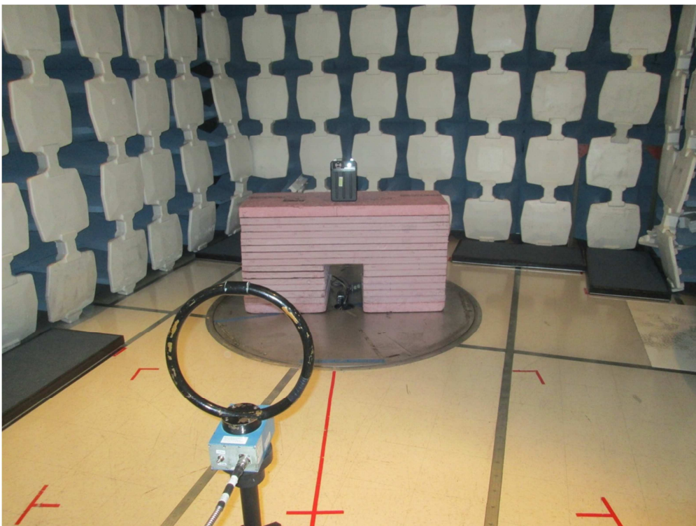
Radiated Spurious Emissions (1MHz - 30MHz)
