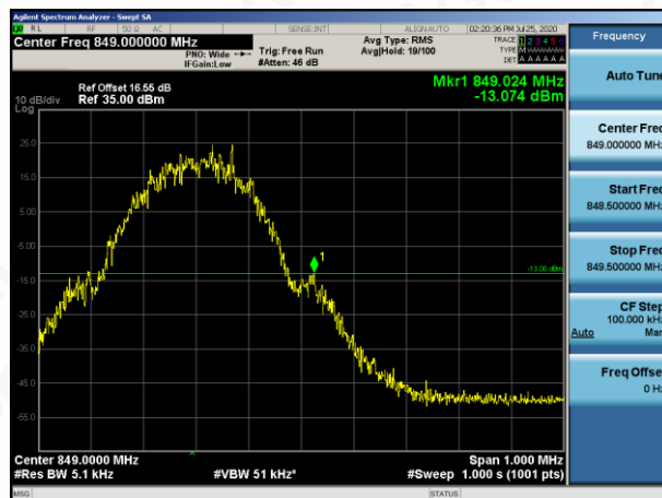
GSM 850-HCH-GSM
